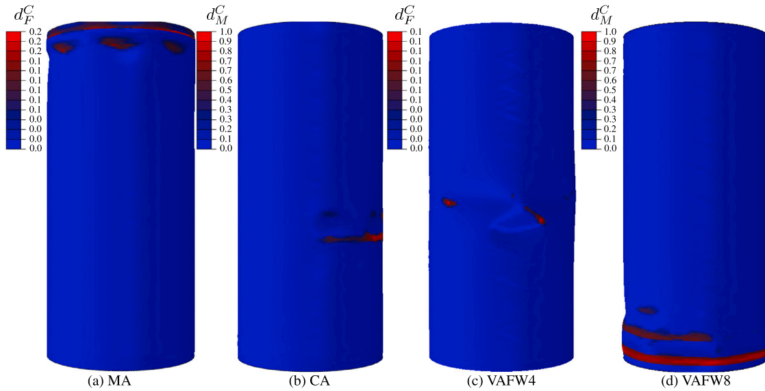
Fig. 16. Plot of the most critical damage mode after failure for every cylinder. (For interpretation of the references to color in this figure legend, the reader is referred to the web version of this article.)
