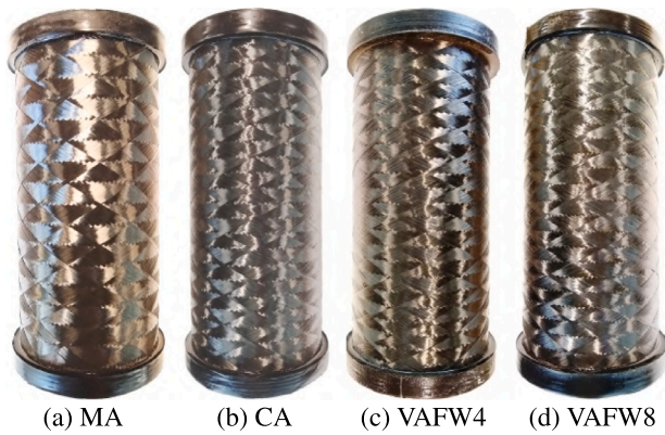
Fig. 6. The prepared cylinders prior to testing.
