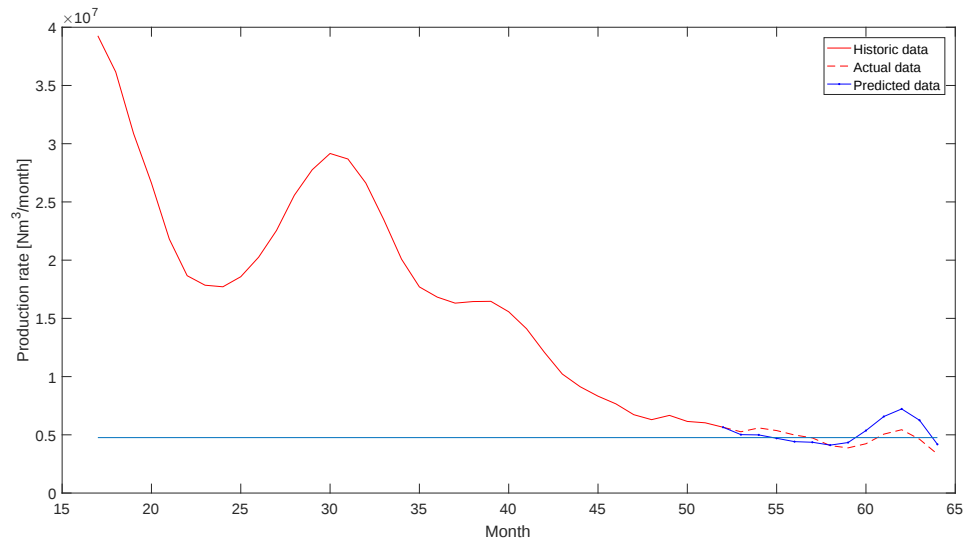
Figure 10: The actual and the predicted flow rate by ANN for well 1. When the well falls below the Coleman Critical rate liquid loading occurs. Each month a new prediction is made until the actual moment of liquid loading is found.
