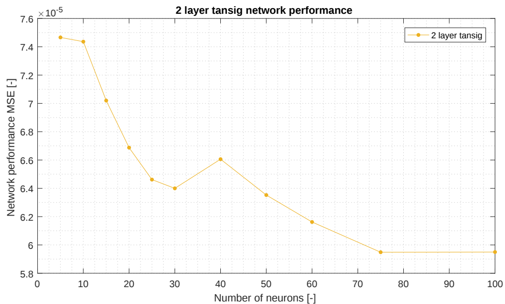
Figure 5.23: Sensitivity analysis based on a 2-layered-tansig-network. 75 neurons show the lowest MSE with a value of 5.9484 \times 10^{-5} and thus the best performance.
