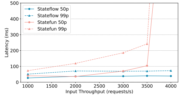
Figure 4: Average and 99th percentile latency for the M workload, with increasing input throughput.
