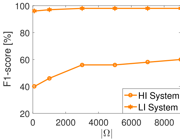
Fig. 10. Prediction performance for different training database sizes.
