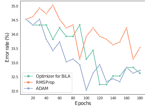
Figure 6: Error rates for different optimizers on Age.
