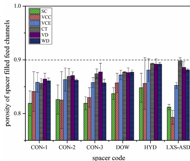
Fig. 4. Comparison of porosities of spacer filled feed channels in MFS for six feed spacers based on porosity methods: volumetric calculations: strand count (SC), cylindrical (VCC) and ellipsoidal (VCE), CT-scan (CT), volume displacement (VD) and weight and density (WD).
