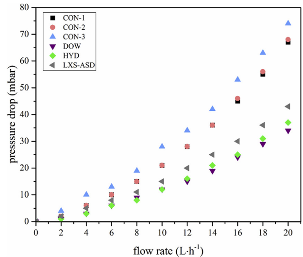
Fig. 6. Feed channel pressure drop (mbar) as a function of feed water flow ( \text{L} \cdot \text{h}^{-1} ) in MFSs for six different feed spacers: CON-1, CON-2, CON-3, DOW, HYD and LXS-ASD.
