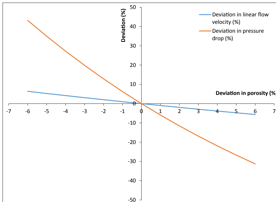
Fig. 5. Effect of feed channel porosity measurement deviation in percent (%) on linear flow velocity and pressure drop for a 34-mil thick standard spacer at a feed flow rate of 16 \text{ L} \cdot \text{h}^{-1} .
