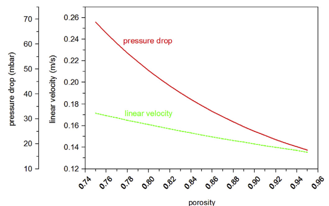
Fig. 1. Linear velocity and pressure drop calculations for a 34-mil (864 \mu\text{m} ) thick standard spacer at a feed flow rate of 16 \text{ L} \cdot \text{h}^{-1} and a feed channel porosity ranging from 0.75 to 0.95.
