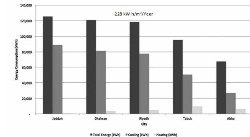
FIG. 2.5 Total annual energy consumption, space cooling and space heating for a villa located in five cities. Source: [29].
