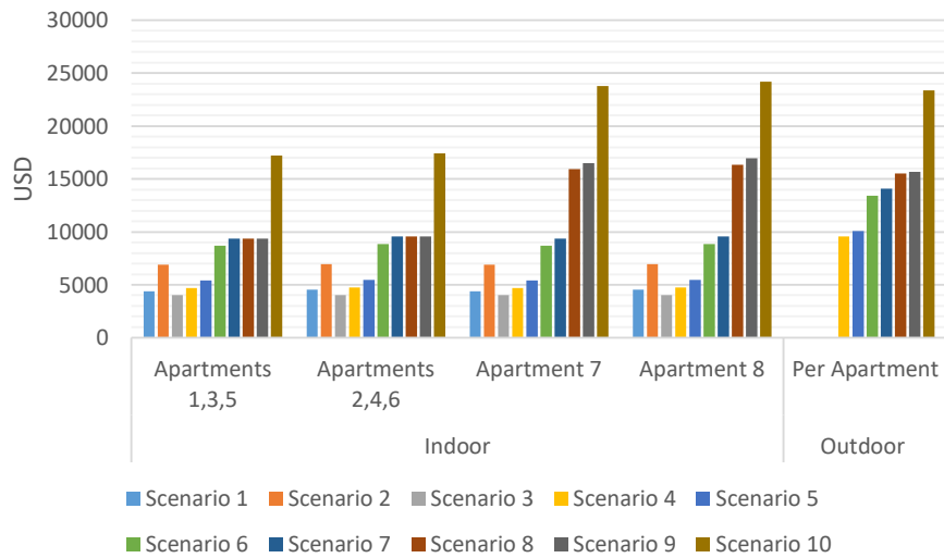
FIG. 5.5 Cost calculation for proposed scenarios for all apartments (indoor and outdoor).
