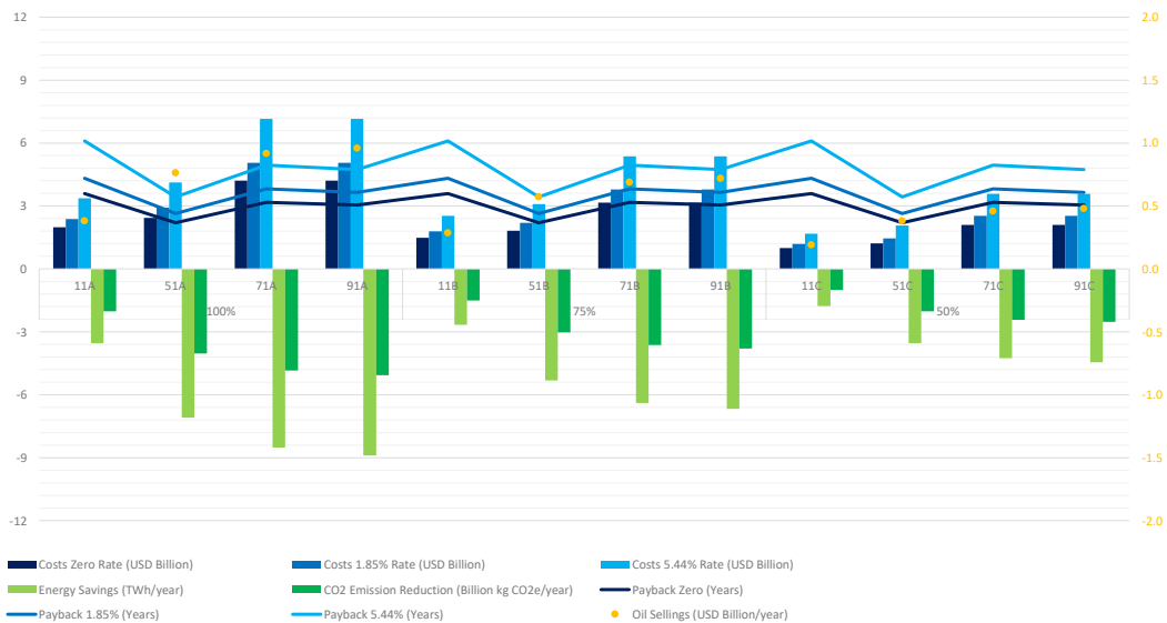
FIG. 6.2 Calculation of key performance indicators (KPIs) for apartment 1 across four selected indoor scenarios.
