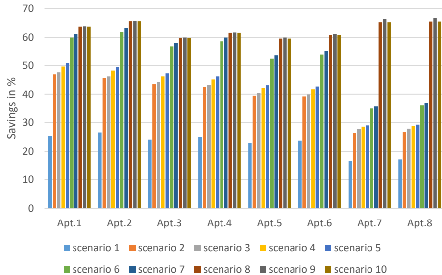
FIG. 4.16 Possible energy savings from testing different scenarios (indoor) where the infiltration rate is 4 ACH50, with a rate of 20 ACH50 for the basic model.
