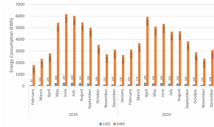
FIG. 3.5 2019-2020 energy consumption and energy cost for 1st floor.
