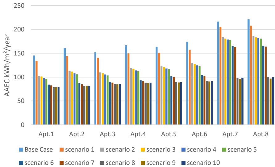
FIG. 4.12 AEC values for indoor energy retrofitting scenarios using 20 ACH50 for infiltration rate, with a rate of 20 ACH50 for the basic model.
