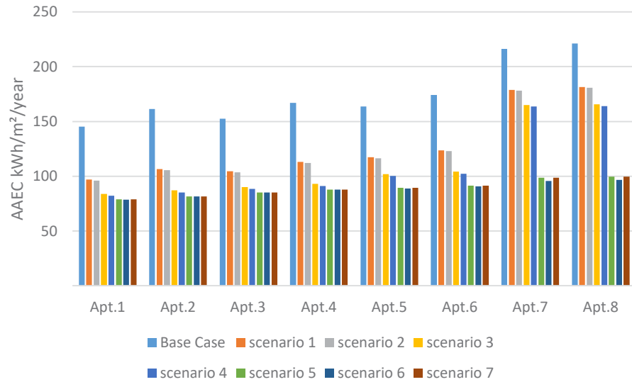
FIG. 4.17 AAEC for outdoor energy retrofitting scenarios using 20 ACH50 for the infiltration rate, with a rate of 20 ACH50 for the basic model.
