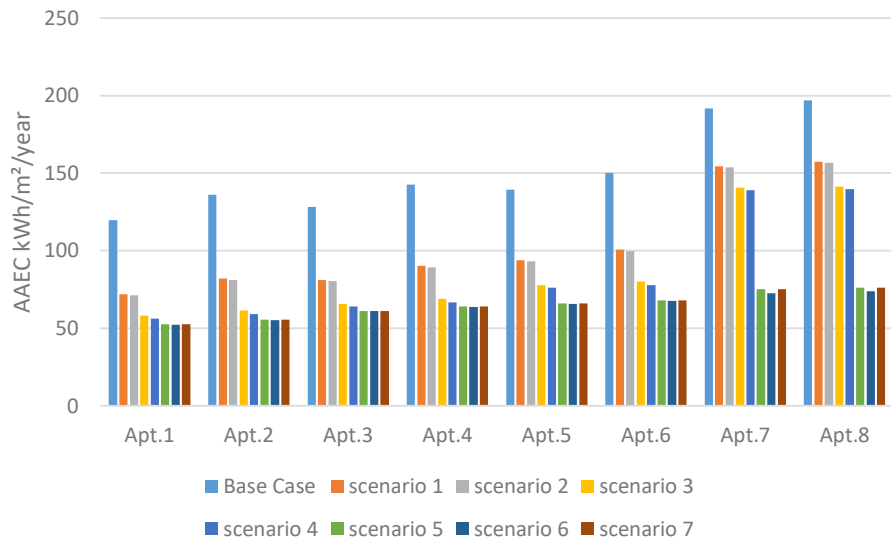
FIG. 4.18 AAEC for outdoor energy retrofitting scenarios using 4 ACH50 for the infiltration rate, with a rate of 4 ACH50 for the basic model.
