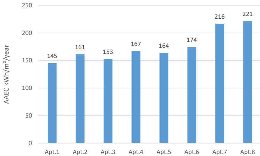
FIG. 5.2 AAEC for 8 apartments in the KSA when the ACH50 is 20.
