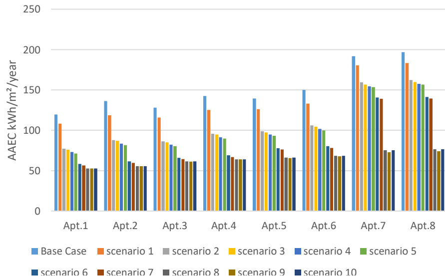
FIG. 4.13 AEC values for indoor energy retrofitting scenarios using 4 ACH50 for infiltration rate, with a rate of 20 ACH50 for the basic model.
