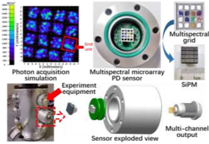
Fig. 1. Multispectral microarray sensor components and optical signal acquisition simulation.
