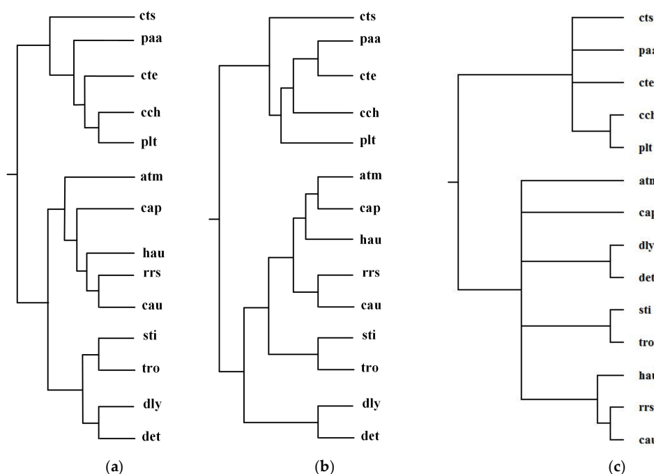
Figure 7. Phylogenetic trees for green sulfur and green non-sulfur bacteria. (a) Our tree T_1 . (b) Ma et al.'s tree T_2 . (c) The NCBI taxonomy T.
