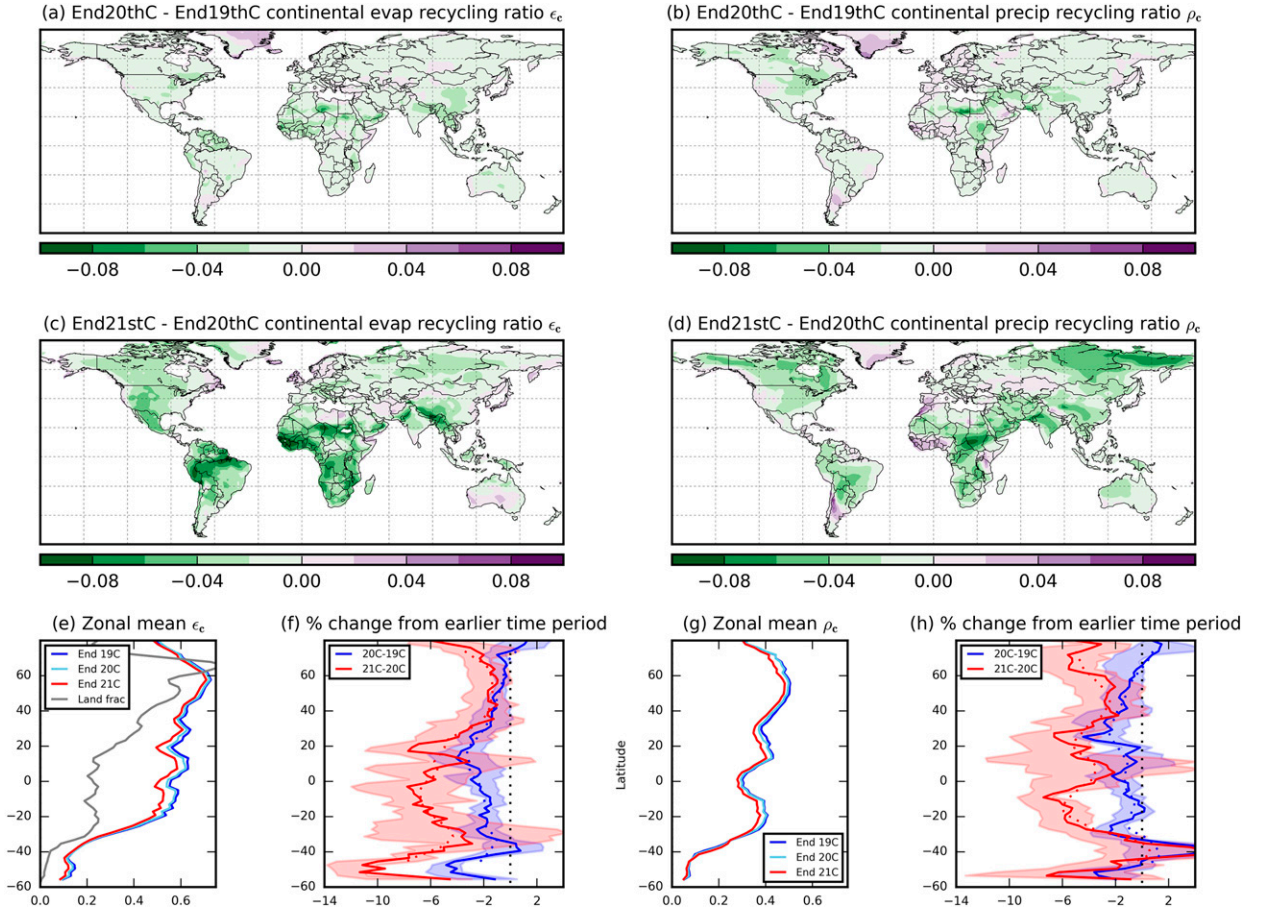
FIG. 3. Differences of average continental (left) evaporation and (right) precipitation recycling ratios (a),(b) between the end of the twentieth and nineteenth centuries and (c),(d) between the end of the twenty-first and twentieth centuries. Also shown are the associated (e),(g) zonal means and (f),(h) zonal mean differences. The shaded areas in (f) and (h) show the 25th–75th percentile ranges of the difference fields across that zonal band. Zonal mean land fraction is also included in (e). South of 20°S, zonal mean ratios decrease rapidly as zonal mean land coverage decreases.
