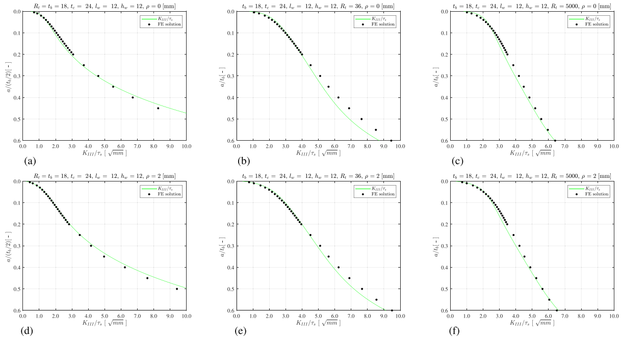
Fig. C.19. Weld toe SIF for \rho = 0 (a-c) and \rho > 0 (d-f) for a DS welded cruciform joint; r_{\tau_1} = 1 (a, d), r_{\tau_1} = 0.25 (b, e), r_{\tau_1} = 0 (c, f).
