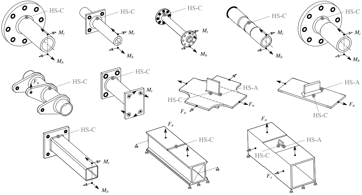
Fig. 9. Fatigue test specimen geometry, external loading (arrows) and constraints (thick lines or \Delta symbols) [21].
