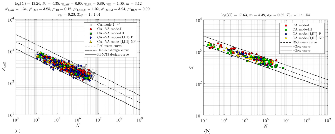
Fig. 15. Effective notch stress based fatigue resistance for uniaxial and multiaxial data and \rho^*_I \neq \rho^*_{\text{III}} , \beta(N) , 1 st order path dependent non-proportionality with c_m = 0.65 (a) and traction equivalent structural stress based fatigue resistance (b).
