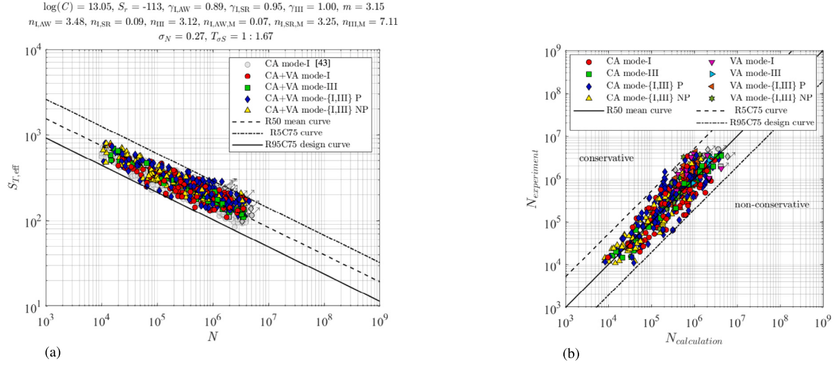
Fig. 14. Total stress based fatigue resistance (a) and lifetime ratio plot (b) for uniaxial and multiaxial data; n_I \neq n_{\text{III}} , \beta(N) , 1 st order path dependent non-proportionality with c_m = 0.40 .
