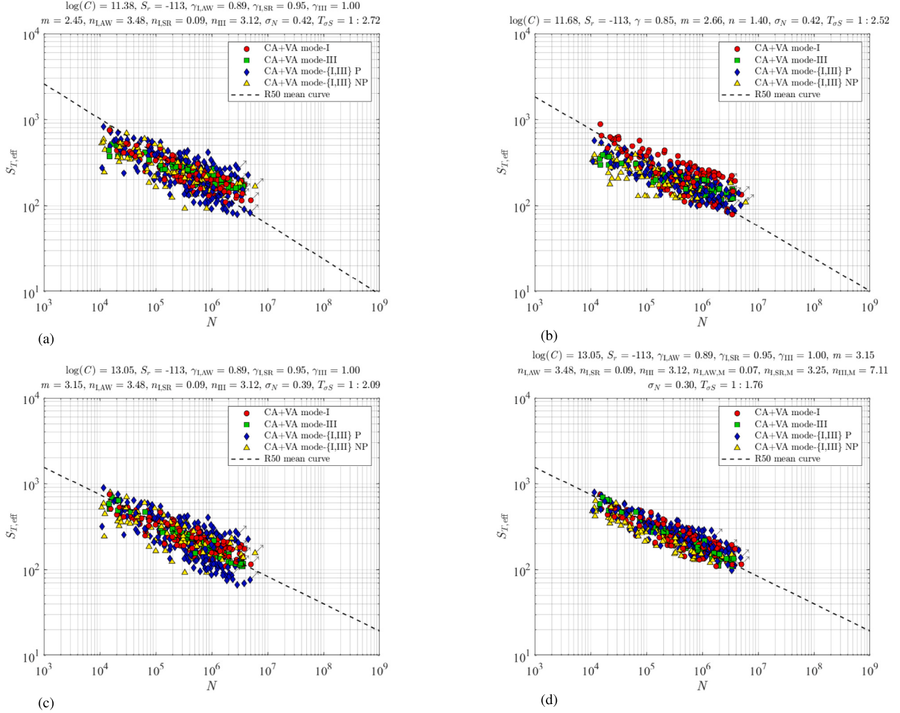
Fig. 11. Total stress based fatigue resistance for uniaxial and multiaxial data adopting: \beta = \sqrt{3} and \{n_I, \gamma_I\} \neq \{n_{III}, \gamma_{III}\} (a); \beta = \sqrt{3} and \{n_I, \gamma_I\} = \{n_{III}, \gamma_{III}\} (b); \beta = f(N) and n_I \neq n_{III} for 3 n approach (c) and 6 n approach (d). Note: c_m = C_{npd} = 0 .
