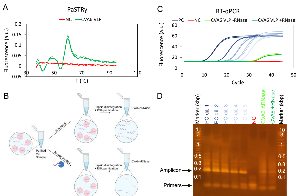
Figure 4.4. RNA presence in CVA6 VLPs.
