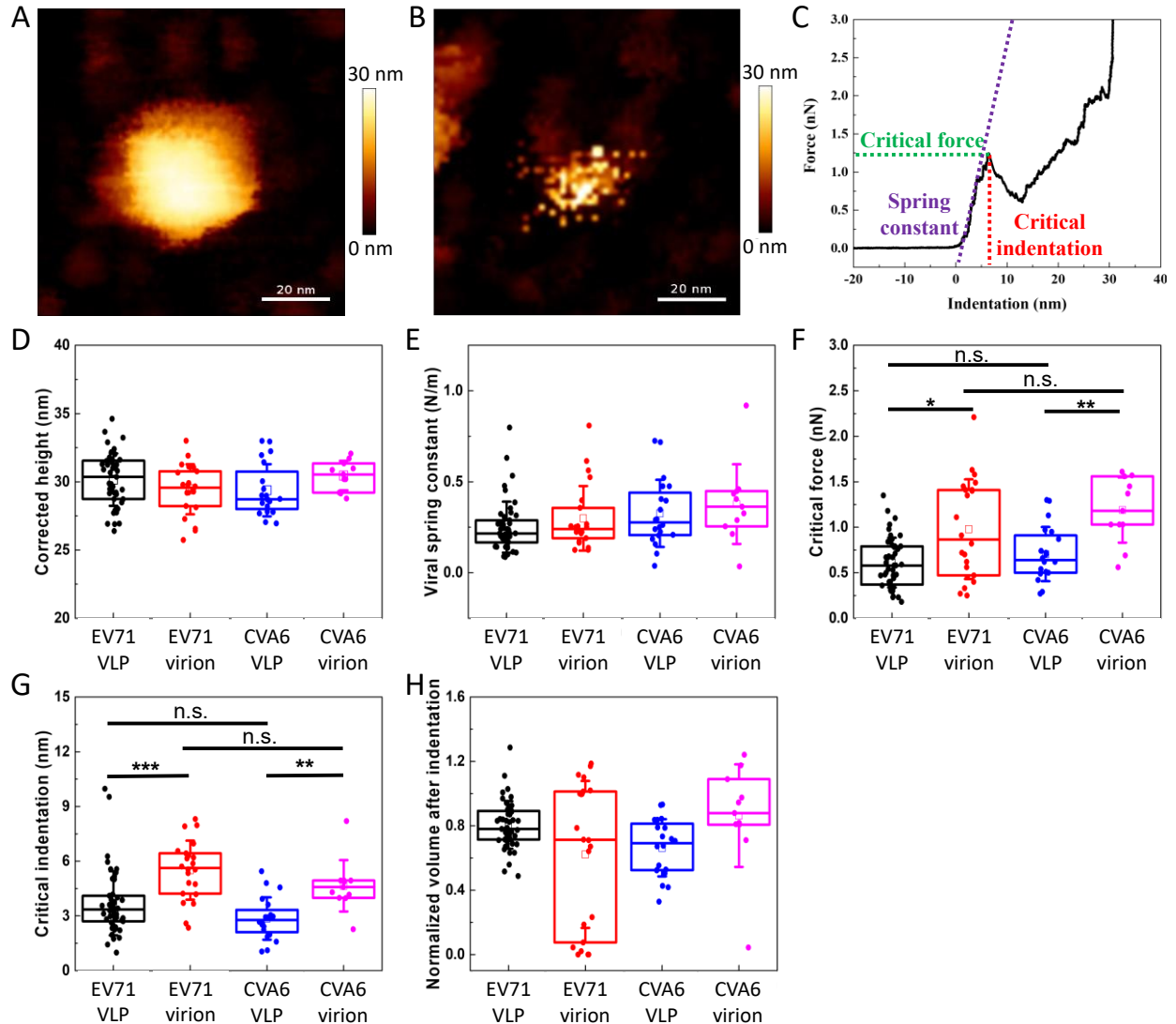
Figure 4.2. AFM results for EV71 VLPs (black), EV71 virions (red), CVA6 VLPs (blue), and CVA6 virions (violet).
