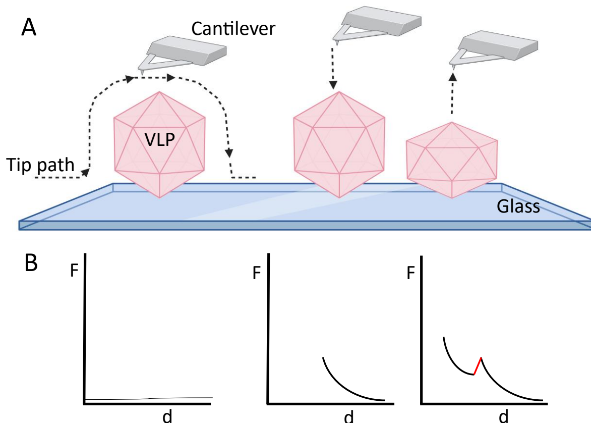
Figure 1.5. Schematic representation of AFM imaging and manipulation.
