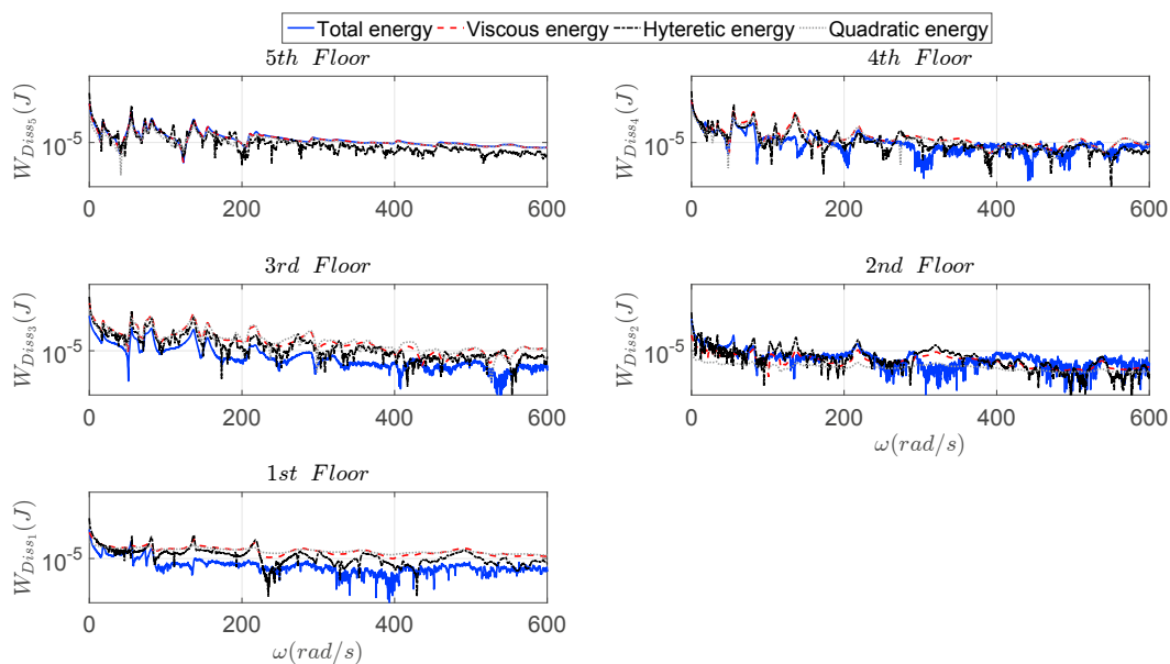
Fig. 6. Comparison of the energy dissipation of the different damping operators at each floor segment
