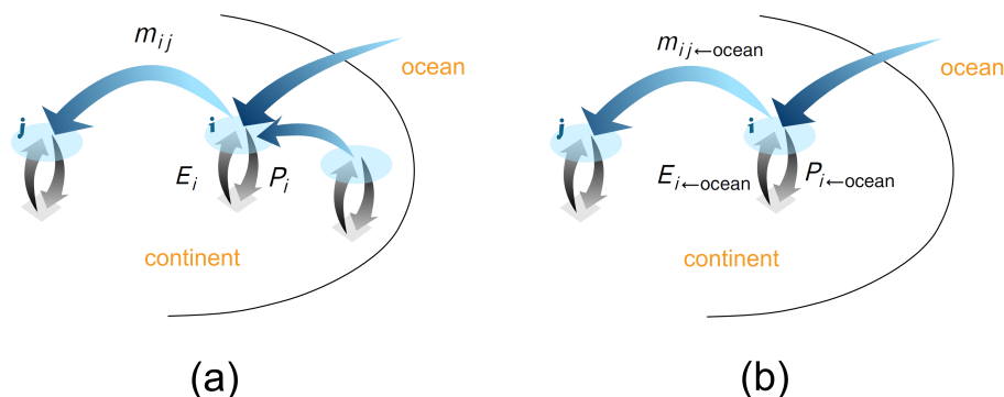
Figure B1. Scheme explaining the removal of CMR. Originally, the precipitation in the grid cell i ( P_i ) is composed of oceanic and continental moisture. The total incoming moisture is evaporated in i ( E_i ) and some part of it contributes to precipitation in the grid cell j ( m_{ij} ) (a). If we forbid the re-evaporation of continental precipitation, only the precipitation in i that has oceanic origin ( P_{i \leftarrow \text{ocean}} ) is evaporated in i ( E_{i \leftarrow \text{ocean}} ) and can contribute to precipitation in j ( m_{ij \leftarrow \text{ocean}} ). By doing so, we remove cascading recycling of continental moisture from the network.
