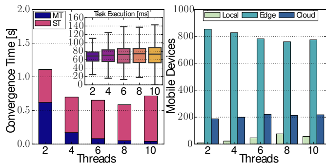
Fig. 13: Performance of 2PMT-Nimbus.
