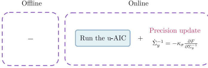
Fig. 2. New fault-tolerant pipeline with precision learning, in contrast to previous work [3] from Fig. 1.
