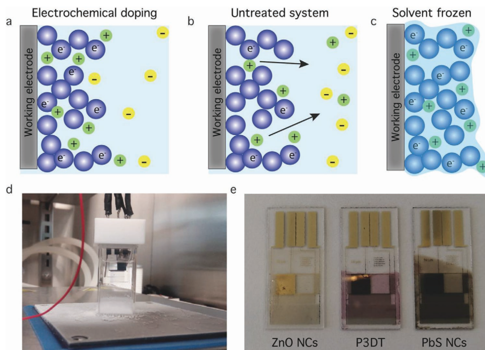
Figure 1. Electrochemical doping of semiconductor films by freezing the electrolyte solvent. a) When a negative enough potential is applied to the working electrode, electron injection takes place. Electrolyte cations diffuse into the voids of the film to neutralize the injected charge. b) When a doped semiconductor film is disconnected from the potentiostat, injected charges disappear. c) By freezing the electrolyte solvent before the potentiostat is disconnected, the doping stability is retained. d) Electrochemical measurement performed at low temperature on a hot/cold plate. e) Semiconductor films used in this study: ZnO NCs, P3DT, and PbS NCs.
