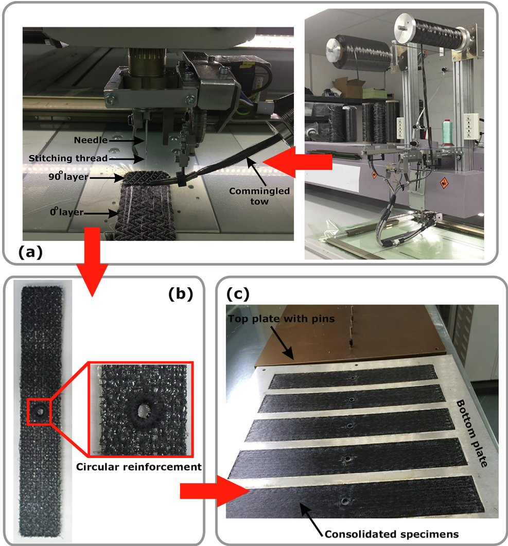
Fig. 3. Manufacturing process: (a) TFP process of the commingled preform at an instance in which a 0° layer is completed while the 90° layer is being placed, (b) one example of a preform showing the circular reinforcement around the hole and (c) consolidated specimens before extraction from the tool.
