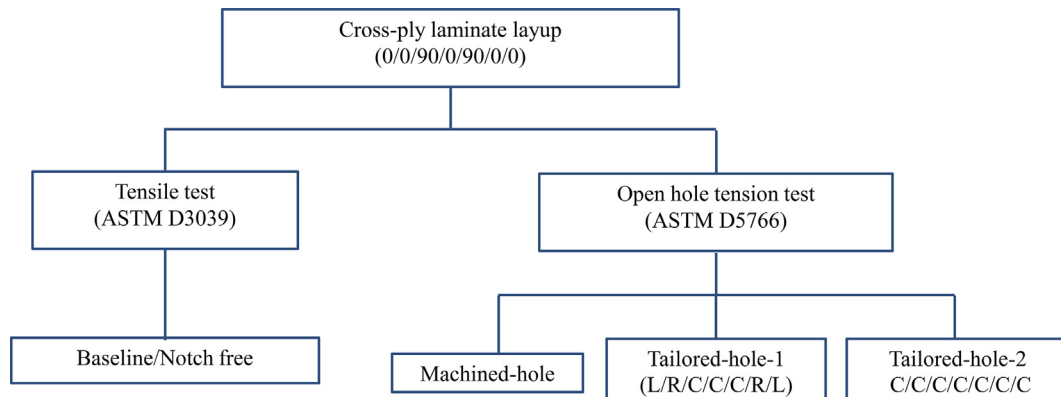
Fig. 2. Schematics of TFP layout of composite samples investigated in this study, C refers to the two central tows steered symmetrically around the hole, L & R are the steered tows from the left and right hand sides of the hole.
