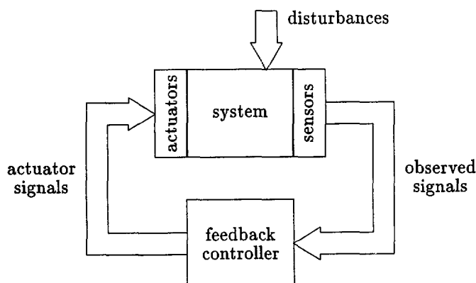
Fig. 1.1: Schematic diagram of a feedback controlled system.
