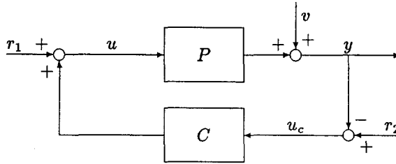
Fig. 2.3: Feedback connection T(P, C) with distinguishable reference signals col(r_2, r_1) and noise signal v .
