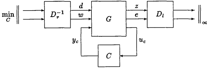
Fig. 5.3: Controller synthesis via \mathcal{H}_\infty optimization for fixed D -scaling.
