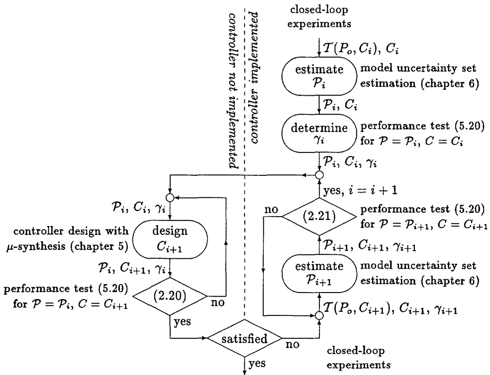
Fig. 7.1: Schematic flow chart of the model uncertainty set estimation, feedback controller design and the controller (2.20) and modelling (2.21) validation test in Procedure 2.5-4.
