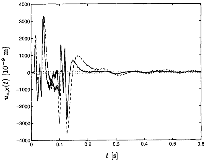
Fig. 8.25: Servo error u_c response to a step in x-direction using controller C_{i+1} (—) and using controller C_i (--) and required accuracy interval (···).
