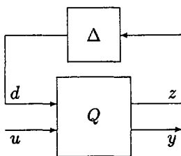
Fig. 5.1: LFT representation of model perturbation.
