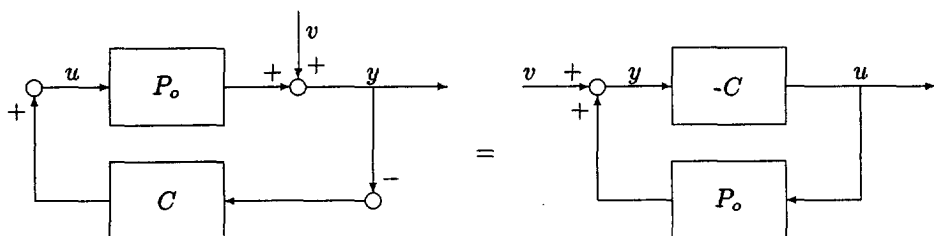
Fig. 3.2: Closed-loop identification without reference signal.
