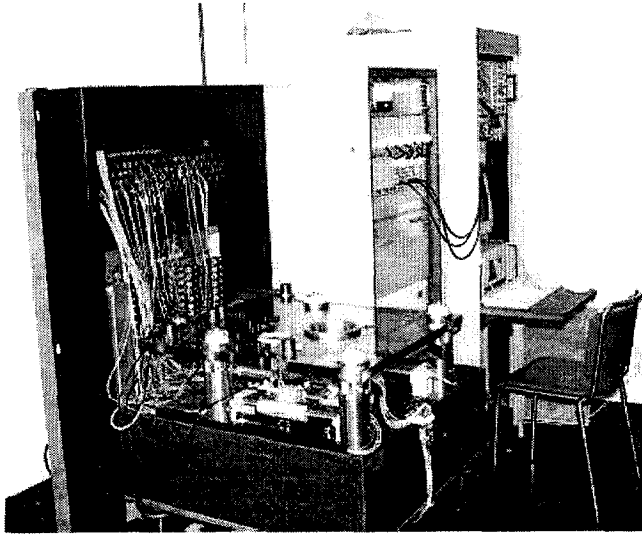
Fig. 8.2: Experimental set up with (from left to right) the wafer stage, interface and host computer with digital signal processor.
