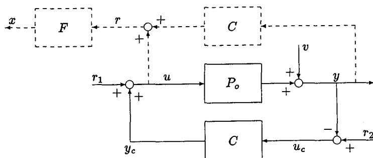
Fig. 4.2: Construction of signal x in (4.24) and admittance to \text{rcf}(N_{o,F}, D_{o,F}) of plant P_o operating in a feedback connection T(P_o, C) .
