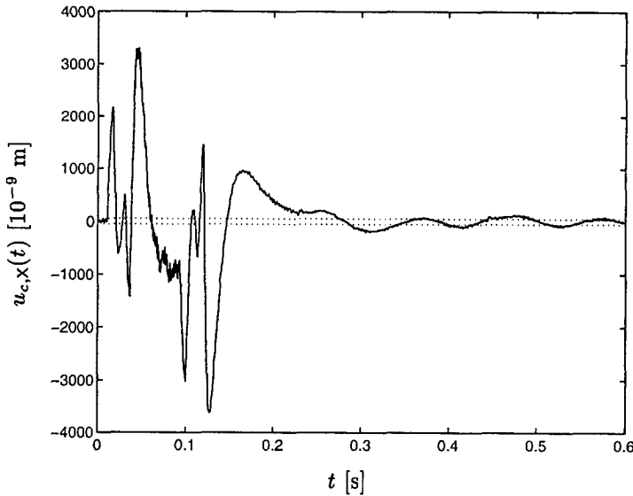
Fig. 8.10: Servo error u_c response to a step in x-direction (—) and required accuracy interval ( \cdots ).
