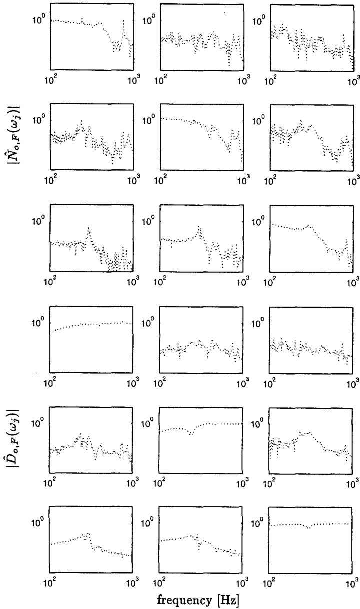
Fig. 8.13: Magnitude Bode plot of experimentally obtained frequency response ( \hat{N}_{o,F}(\omega_j) , \hat{D}_{o,F}(\omega_j) ) of the rcf(N_{o,F}, D_{o,F}) of the plant P_o .
