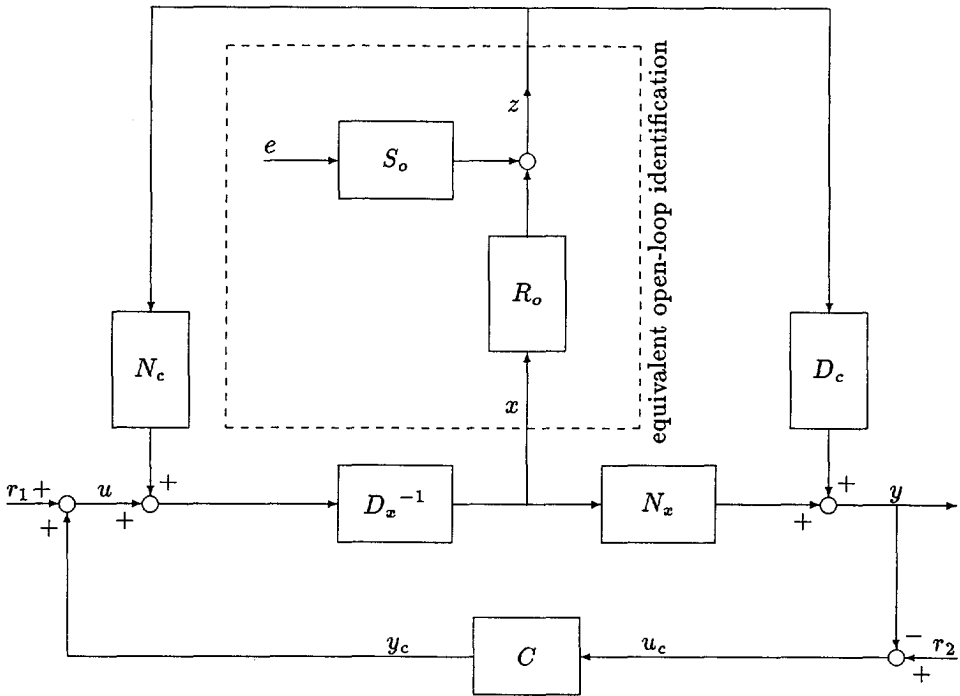
Fig. 4.1: Block diagram of the reparametrization of plant P_o and noise filter H_o given in (4.18).
