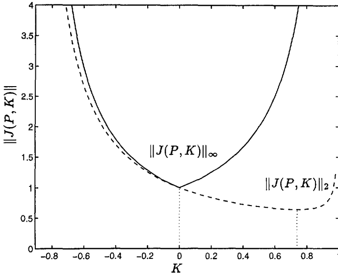
Fig. 2.4: Evaluation of a performance cost over a set of admissible controllers \mathcal{C} . In this plot, J(P, K) = (1 + KP)^{-1} , where the system P is defined in (2.7) and \mathcal{C} is given in (2.8).
