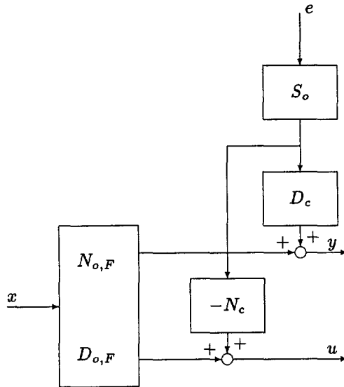
Fig. 4.3: Equivalent open-loop identification of the \text{rcf}(N_{o,F}, D_{o,F}) of the plant P_o using the signal x of (4.24) and the closed-loop data \text{col}(y, u) .
