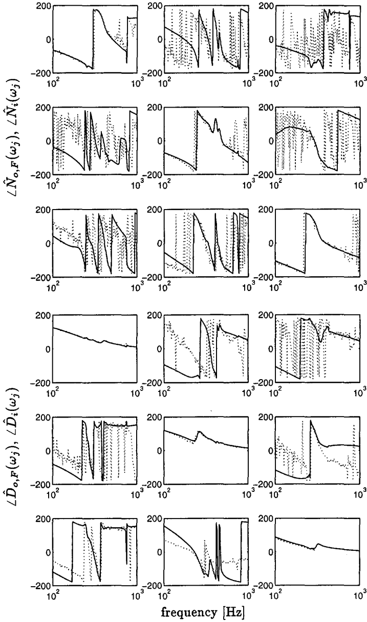
Fig. 8.15: Phase Bode plot of spectral estimate ( \hat{N}_{o,F}(\omega_j), \hat{D}_{o,F}(\omega_j) ) ( \cdots ) and 27th order nominal factorization ( \hat{N}_i(\omega_j), \hat{D}_i(\omega_j) ) (—).
