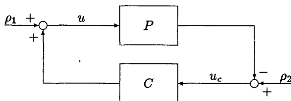
Fig. 2.2: Feedback connection T(P, C) of system P and a controller C .
