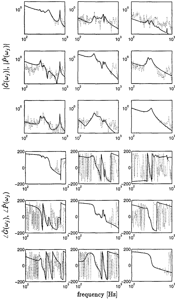
Fig. 8.16: Magnitude Bode plot (top nine plots) and phase Bode plot (bottom nine plots) of spectral estimate \hat{G}(\omega_j) = \hat{N}_{o,F}(\omega_j) \hat{D}_{o,F}^{-1}(\omega_j) ( \cdots ) and 27th order nominal model \hat{P}_i(\omega_j) = \hat{N}_i(\omega_j) \hat{D}_i^{-1}(\omega_j) (—).
