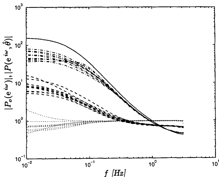
Fig. 3.3: Amplitude Bode plots of plant P_o(e^{i\omega}) (—) and 10 realizations of OE-models P(e^{i\omega}, \hat{\theta}) being estimated for noise intensity \lambda = 5 ( \cdots ), \lambda = 1 ( - - ) and \lambda = 0.2 ( - \cdot - ).
