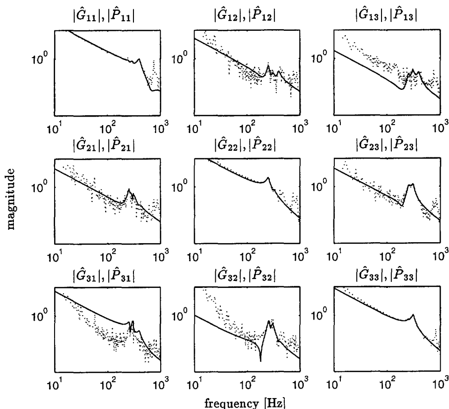
Fig. 8.8: Magnitude Bode plot of experimentally obtained frequency response \hat{G}(\omega_j) ( \cdots ) and 18th order linear model \hat{P} ( — ) found by curve fitting from [de Callafon et al. , 1996].
