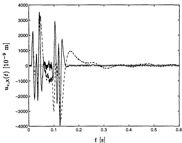
Fig. 8.28: Servo error u_c response to a step in x-direction using controller C_4 (—) and using (initial) controller C_i (- -) and required accuracy interval (···).
