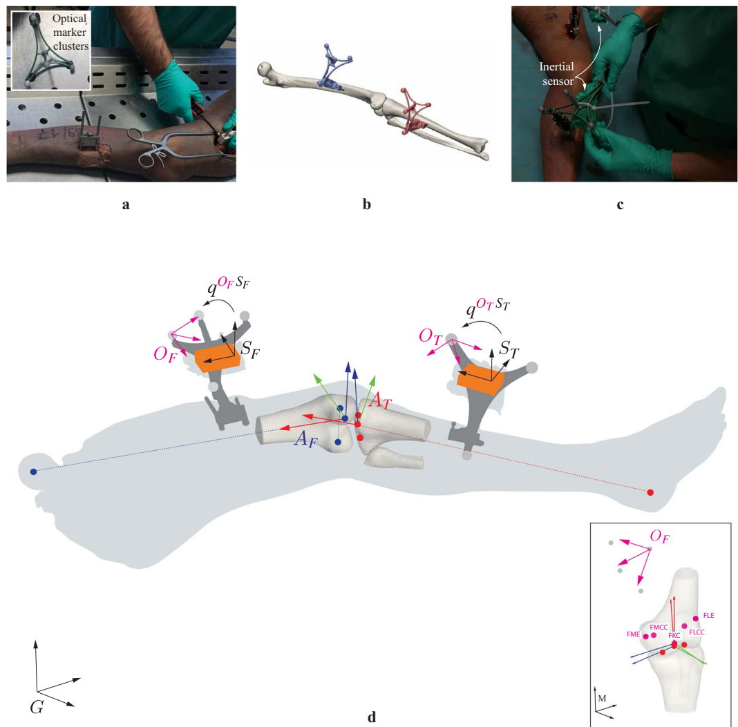
Fig. 1 Experimental set-up. (a) A cadaveric lower limb is equipped with rigidly attached bone-pins, at the medial side of the femur ( _F ) and tibia ( _T ) segments. Each bone-pin is equipped with retro reflective marker clusters (that are used to create optical marker-based coordinate systems O_F and O_T ) and inertial sensors (orange boxes) with sensor coordinate systems S_F and S_T . (b) Three-dimensional surface bone models are reconstructed for the femur and tibia bone and osseous anatomical landmarks are identified within Mimics. Anatomical reference coordinate systems A_F and A_T are defined on the base of virtual anatomical landmarks. Anatomical landmarks are furthermore rotated into a common intermediate coordinate system (pink) within the CT-scan coordinate system M , to rotate the landmarks into the optical motion capture reference frame G . The full explanation of all abbreviations of the annotated anatomical landmarks can be found in Table 1. (c) Inertial sensor are rigidly attached on the femur and tibia-attached bone-pins via zip ties. The alignment rotations q^{O_F S_F} and q^{O_T S_T} define the rotation from coordinate frame S to coordinate frame O for the femur and tibia-attached inertial sensors. As a result, all coordinate systems can be tracked with respect to the optical motion capture reference coordinate system G , after the necessary coordinate system transformations. (d) Illustration of the measurement set-up with the different coordinate frames.
