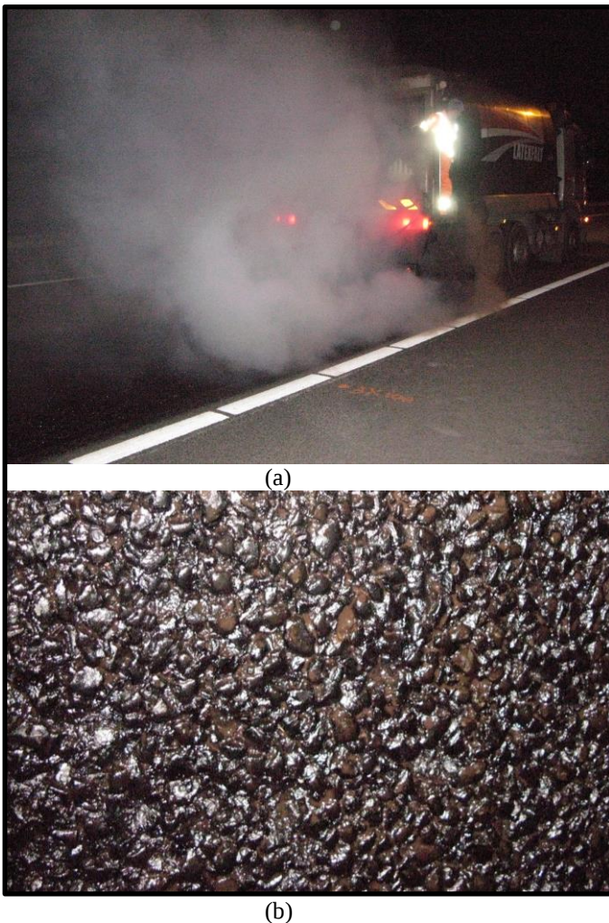
Fig. 10: Application of rejuvenator (a, top) and the PA surface after application (b, bottom)
