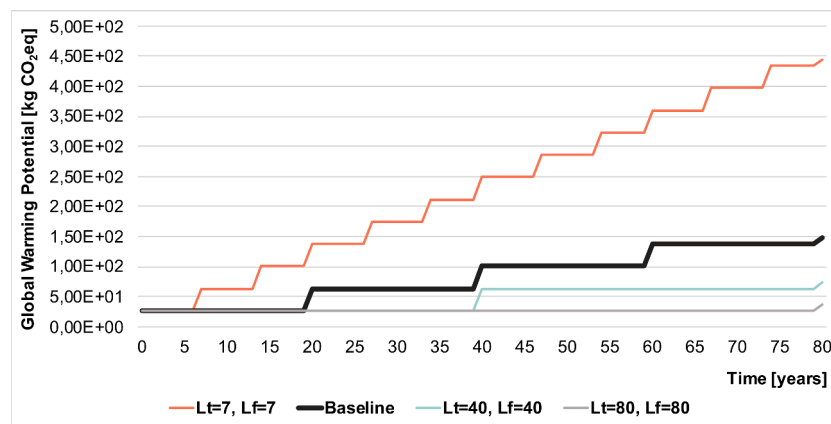
Fig. A6.2a. Sensitivity analysis on the L_{\text{technical}} and L_{\text{functional}} for the BAU kitchen (GWP over 80 years).
