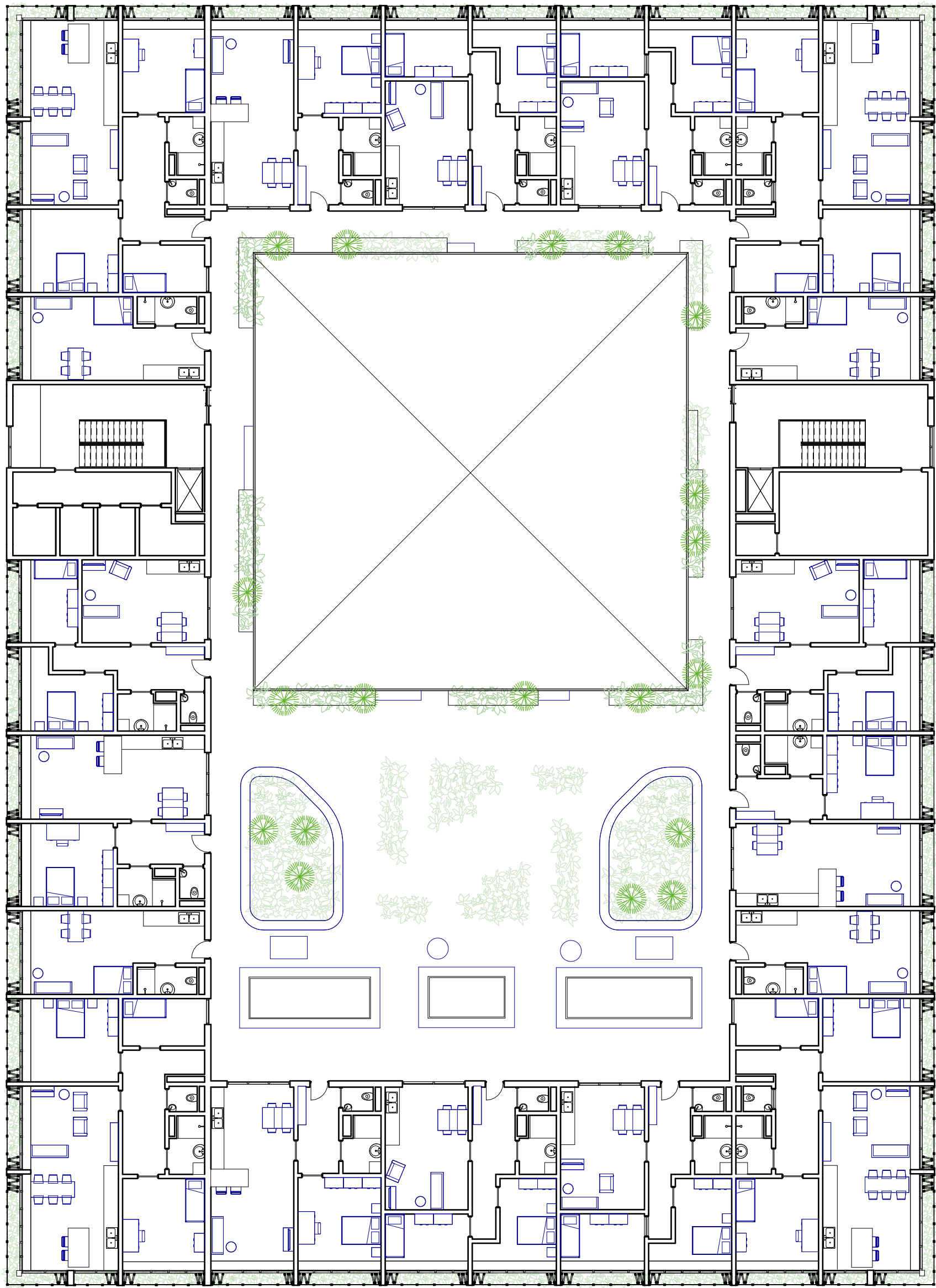
Second floor
