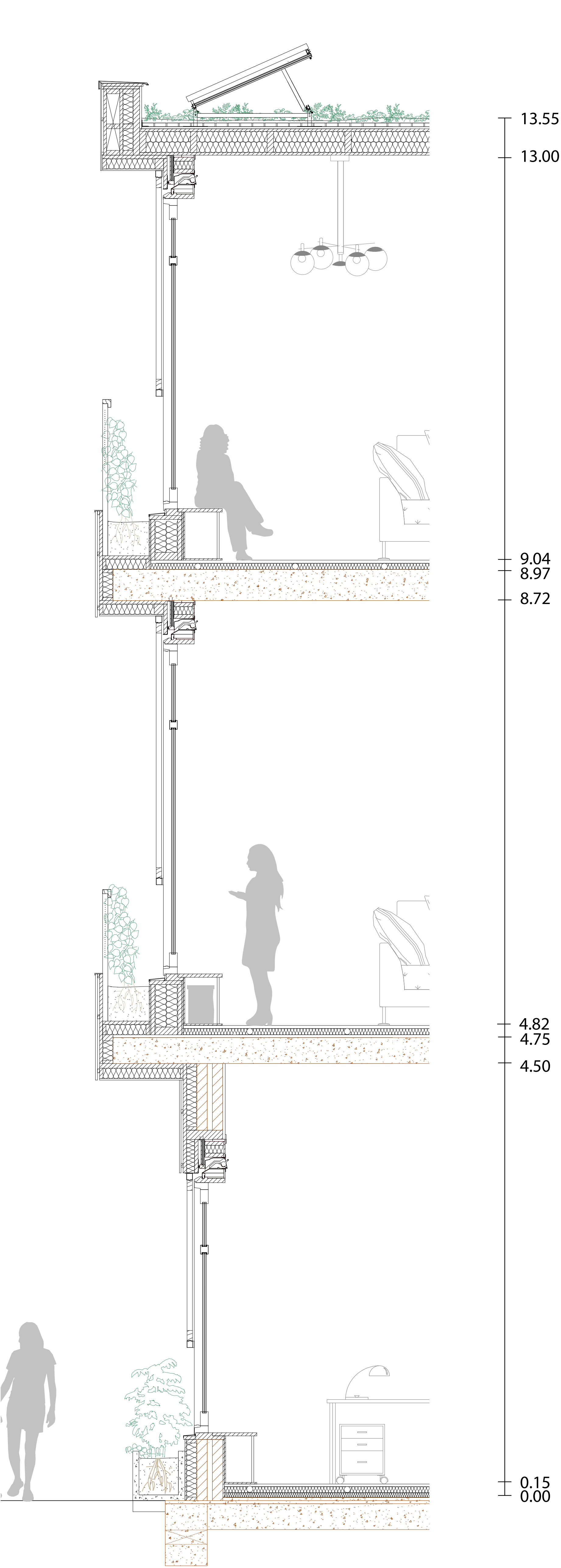
Section fragment 1:20
