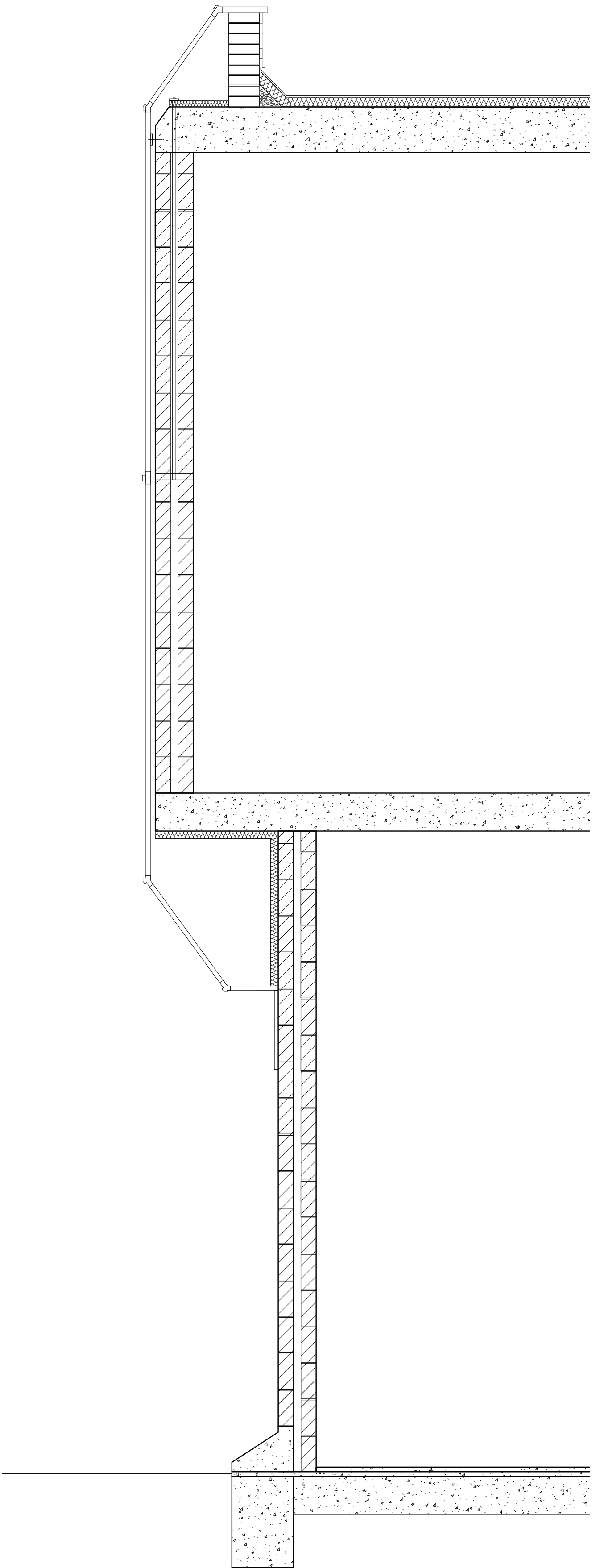
Section fragment 1:20
