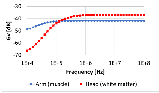
Fig. 4: Voltage gain in muscle [16] and white matter
