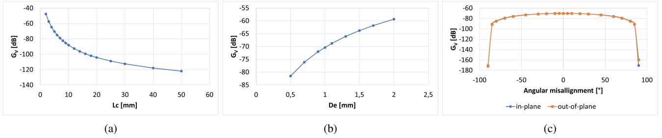
Fig. 6: Voltage gain peak for different a) channel lengths, b) inter-electrode distances, and c) angular misalignments
