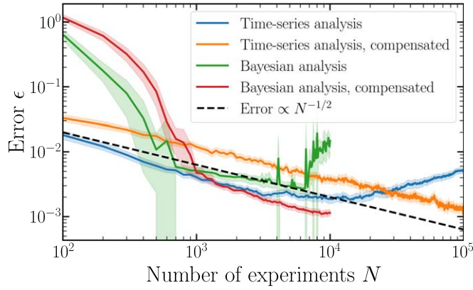
Figure 7. Convergence of Bayesian and time-series estimators in the presence of depolarizing noise and multiple eigenvalues, both with and without noise compensation techniques (described in text). Fixed parameters for all plots are given in text. Shaded regions denote a 95% confidence interval (data estimated over 200 QPE simulations). The black dashed line shows the N^{-1/2} convergence expected in the absence of sampling noise. Data for the Bayesian estimator was not obtained beyond N = 10^4 due to computational constraints.
