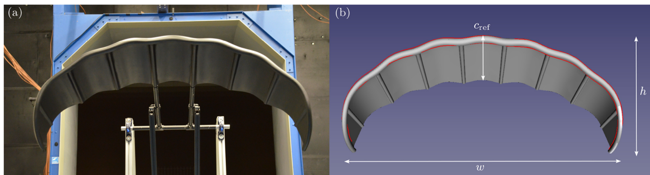
Figure 3. Rigid-scale model of the TU Delft LEI V3 kite. (a) Photograph of the model, rotated by 180^\circ , with its back facing the blue octagonal OJF exhaust nozzle. (b) Rendering of the model from a similar perspective, with the laser-tracked outline overlaid in red and the reference chord c_{\text{ref}} , height h , and width w indicated in white.
