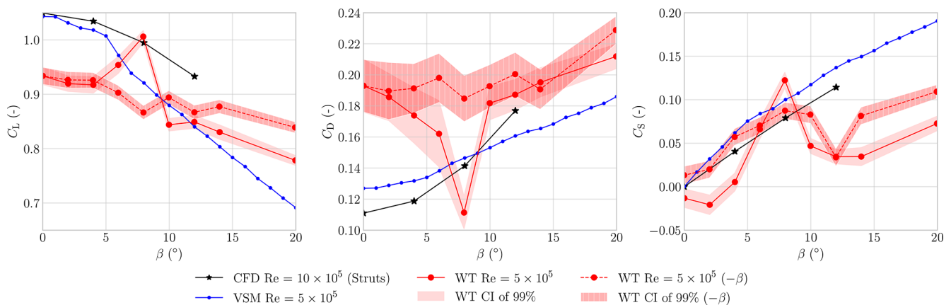
Figure 11. Measured lift, drag, and side force coefficients, together with coefficients computed with VSM and RANS CFD (Viré et al., 2022), plotted against \beta , for \alpha = 12.5^\circ .
