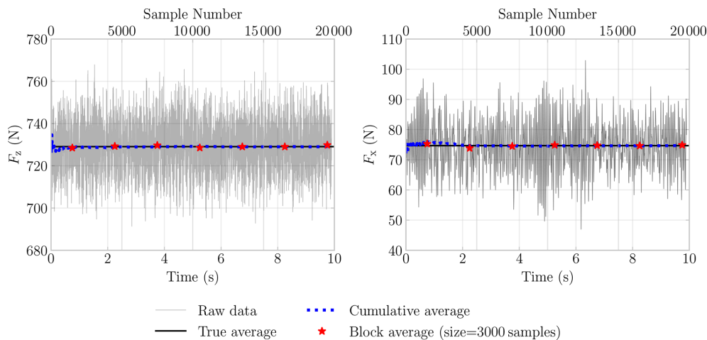
Figure A1. Running average and block average analyses of the 10 s over a sample showing the forces in the z and x axes, demonstrating that the selected period is sufficiently long to achieve a statistically converged average.
