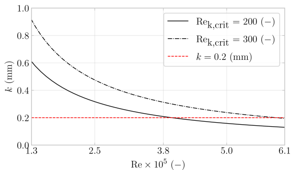
Figure 6. Required minimal trip height vs. Re for different values of Re_{k,crit} .
