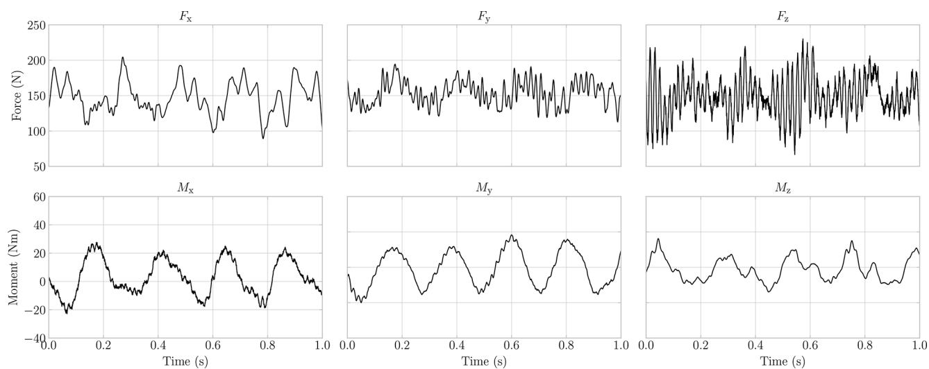
Figure E1. Raw measured values at 2000 Hz by the load balance, over a 1 s period taken at 25 \text{ m s}^{-1} with \alpha = 15^\circ and \beta = 0^\circ .
