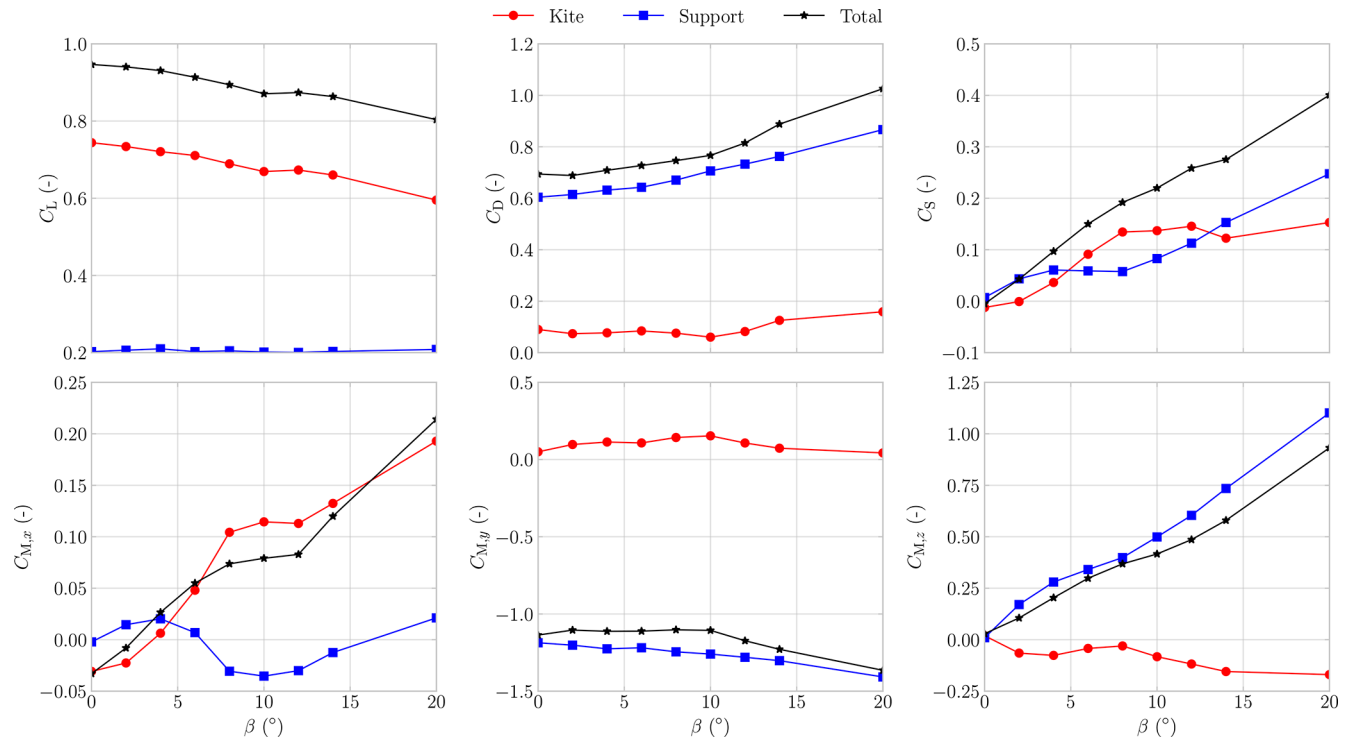
Figure D1. Total measured, support-structure-measured, and kite-measured loads plotted for Re = 5 \times 10^5 over a positive \beta sweep for \alpha = 7.4^\circ .
