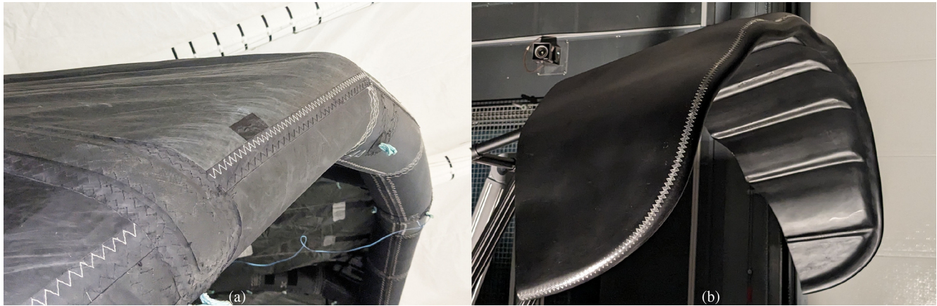
Figure 5. (a) Kitepower V3.25B kite with seams along the leading edge. (b) Scale model with zigzag tape applied to the leading edge. Although they have slightly different designs, the V3.25B and TU Delft V3 kites are practically identical with respect to the flow over the wing's suction side.
