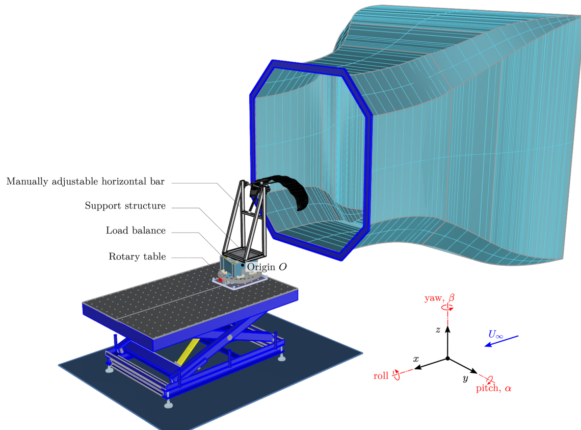
Figure 2. CAD drawing of the experimental setup, showing the origin O in the load balance representing the point at which the load measurements are made. With a sideslip angle \beta = 0^\circ , the x axis runs along the longitudinal direction of the wind tunnel, pointing downstream parallel to the wind. The y axis is oriented laterally, pointing to the right when facing upstream, or, from the kite's perspective, right when looking from the trailing edge towards the leading edge. The z axis is vertical, pointing upwards. The rotary table, load balance, support structure, and kite are all placed on the blue table, which was adjusted in lateral position and height to centre the model in the nozzle exit.
