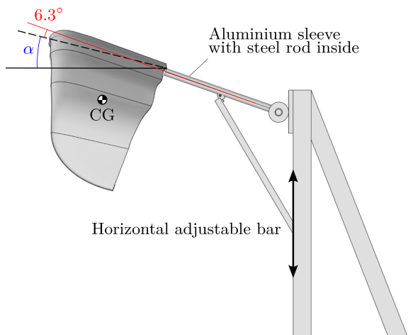
Figure 4. Manual setting of the scale model’s angle of attack with respect to the inflow by adjusting the vertical position of the strut attachment to the support structure. The centre of gravity of the scale model is indicated by point CG.
