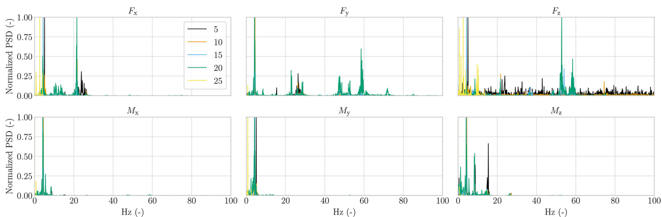
Figure E2. Raw measurements transformed into PSD using FFT and a periodogram function and displayed for the three force and moment components up to 100 Hz.
