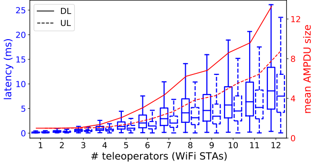
Fig. 4: Plot showing UL and DL latency and corresponding mean AMPDU size over a range of teleoperators (WiFi STAs) for vanilla WiFi-7 implementation.
