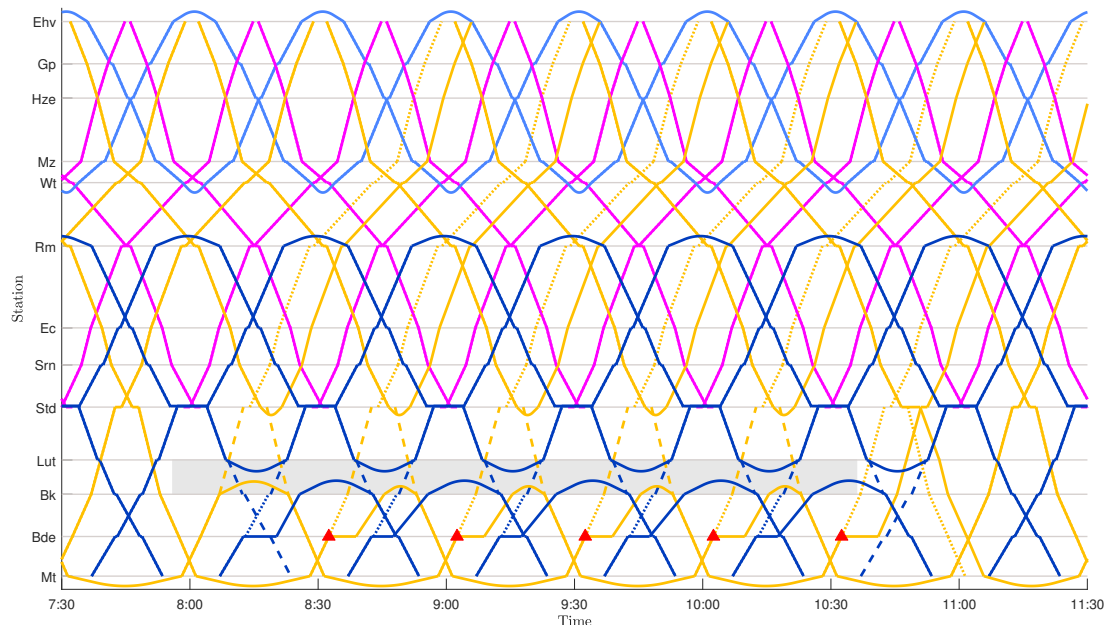
Figure 4.10: The rescheduled timetable by the stochastic approach at stage 2 in case II (disruption end time: 10:36)
