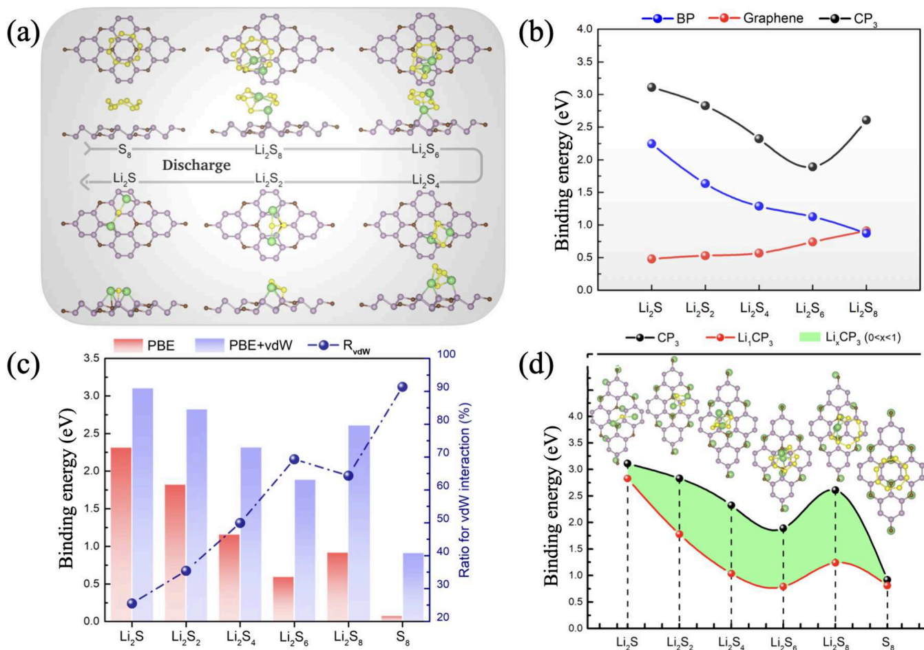
Figure 3. (a) The top and side views of the fully optimized structures of S_8/Li_2S_n molecules on CP_3 monolayer. (b) Computed binding energies of Li_2S_n molecules on blue phosphorene, graphene, and CP_3 monolayers. (c) Computed binding strengths of S_8/Li_2S_n molecules on CP_3 monolayer through DFT and DFT-D3 correction and their corresponding ratio ( R_{vdW} ). (d) Computed binding energy with different Li-concentrations on the CP_3 monolayer.
