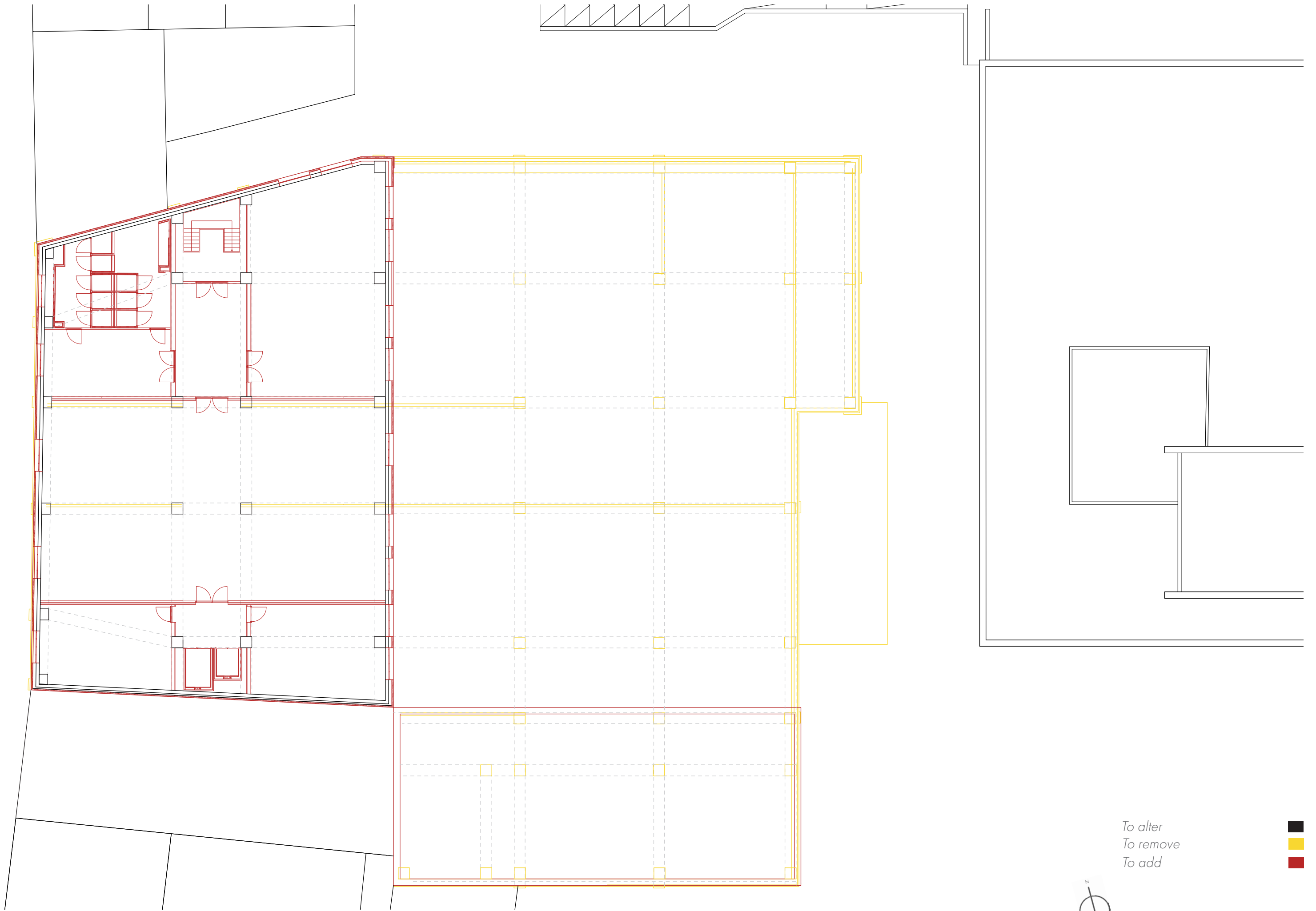
First floor plan, demolition plan
