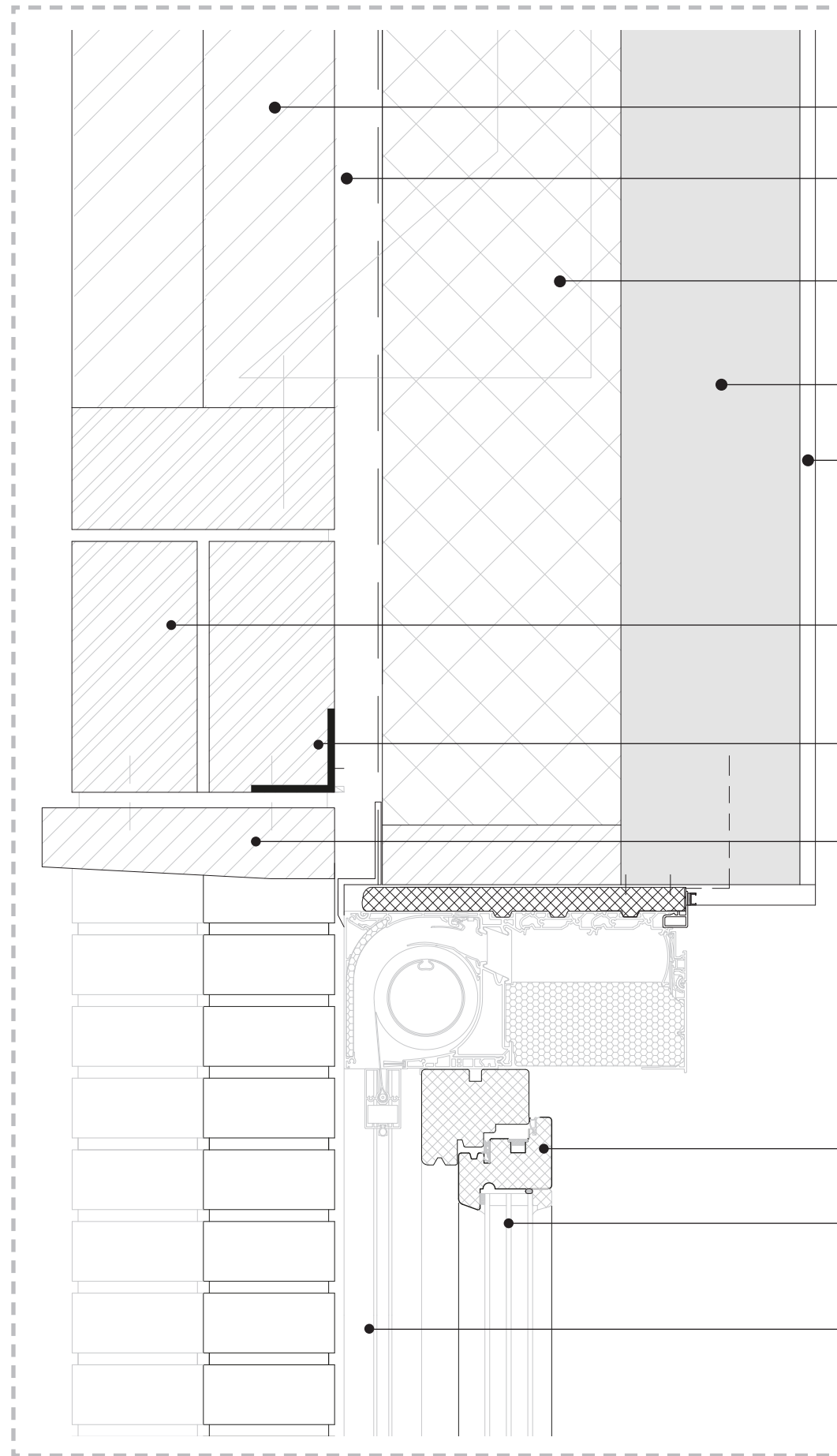
Window element (Upperpart), Detail 1.5
