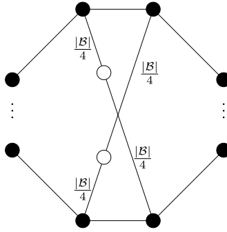
Fig. 3. Instance for which inequality of Lemma 1 is asymptotically tight for c = 2 , where \mathcal{B} is the set of black (non-white) vertices.
