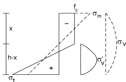
Fig. D-7. Loading lines and ultimate bending stress diagram on semi-full-scale glulam beams with the theoretically necessary perfect boundary conditions of the supports. There always occurred damage through lateral buckling, as follows from the cracking sounds during loading and the decreased (lateral) modulus of elasticity after unloading, even after the smallest possible lateral displacements and even for the most slender beams. The theory of elasticity in Chen and Atsuta (1972) does not show bifurcation for the three dimensional lateral buckling case, and the large displacements analysis (third order theory) shows a continuous rise in the loading curve (see fig.D-7). This means that the top of a loading curve always is due to damage and failure and therefore elastic buckling does not exist in praxis for the applied full size structural elements, as confirmed by the tests.
