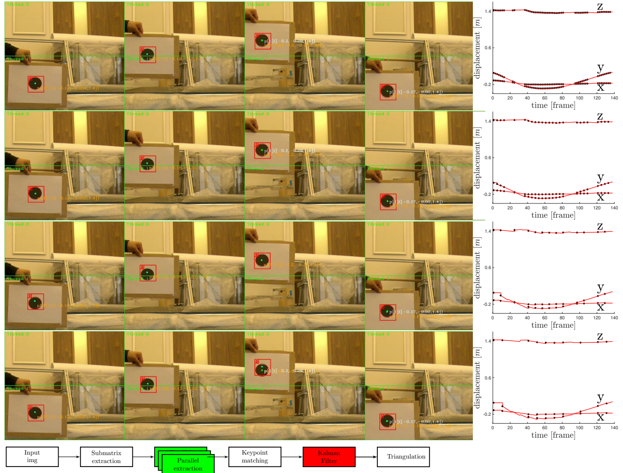
Figure 9 Tracking sequence on input images from left camera (11,30,60,120) for experimental conditions F2-F10 with longer Kalman prediction intervals and reduced frequency of keypoint matching and extraction. Rows 1-4 correspond to the conditions F2,F4,F8 and F10, the last column shows the reconstructed motion in X, Y, Z from Kalman predictions of the two image pairs and the available measurements (black dots).
