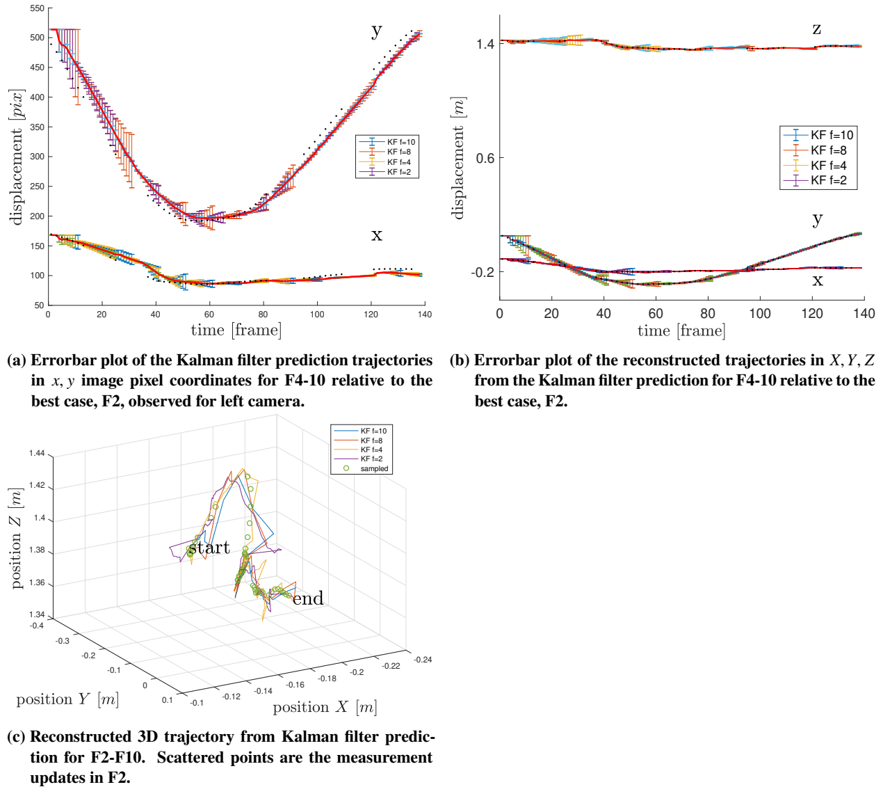
Figure 10 Trajectory reconstruction of the Kalman filter predictions for F2-F10
