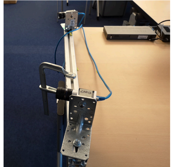
(b) Close up of the stereo camera setup
