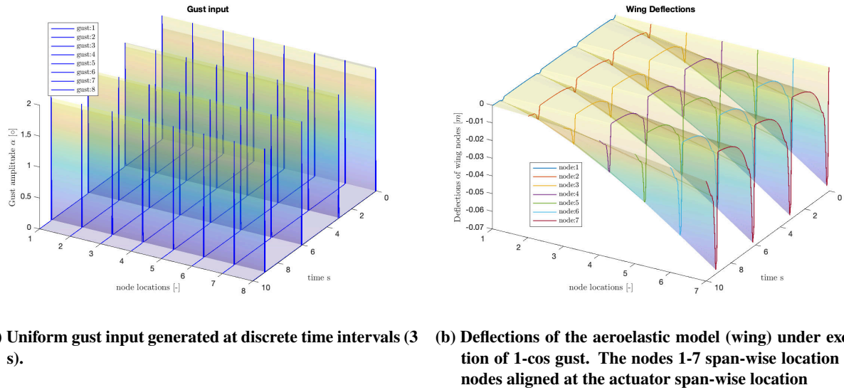
Figure 11 The input and output response of the aeroelastic model for the duration of 10 seconds.
