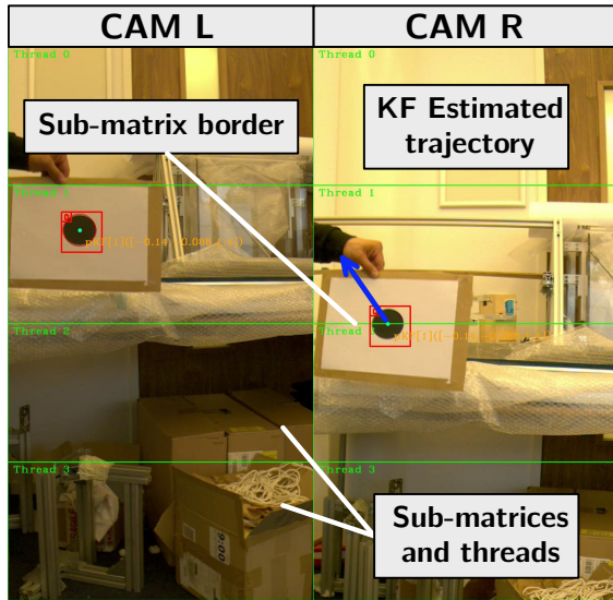
(a) Experimental testing of the parallel 3D reconstruction pipeline. The left and right images correspond to camera 1 and 2 respectively. The images shown the Kalman filtering process when the keypoints switches sub-matrix domain (border transition)
