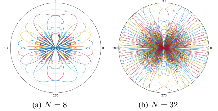
Fig. 3: The beam pattern of uniform linear array antennas.
