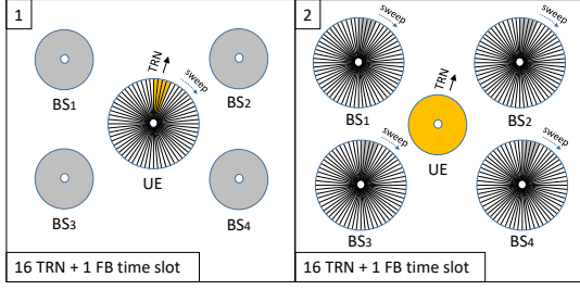
Fig. 5: Parallel fully-sweep beam training.
