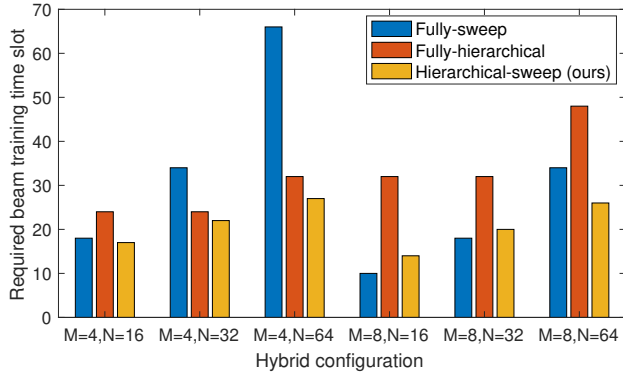
Fig. 8: Required time slots on beam training.
