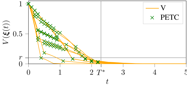
Fig. 3. Trajectory of the Lyapunov function for 10 different initial conditions under MPETC, with PETC samples marked. The maximum time T^* it takes to reach \mathcal{X}_P = r\mathcal{X}_0 is highlighted.
