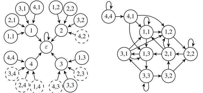
Fig. 1. On the left, an illustration of \mathcal{S}^S (all states) and \mathcal{S}^B (only solid-line states). On the right, a depiction of \mathcal{S}^S with \mathcal{X}^{S'} = \{\sigma \in \mathcal{X}^B : |\sigma| = 2\} .
