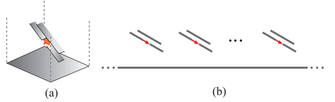
Fig. 1. Array of titled stacked dipole elements, in the presence of an infinite ground plane: (a) 3D-view of the unit cell and (b) side view.
