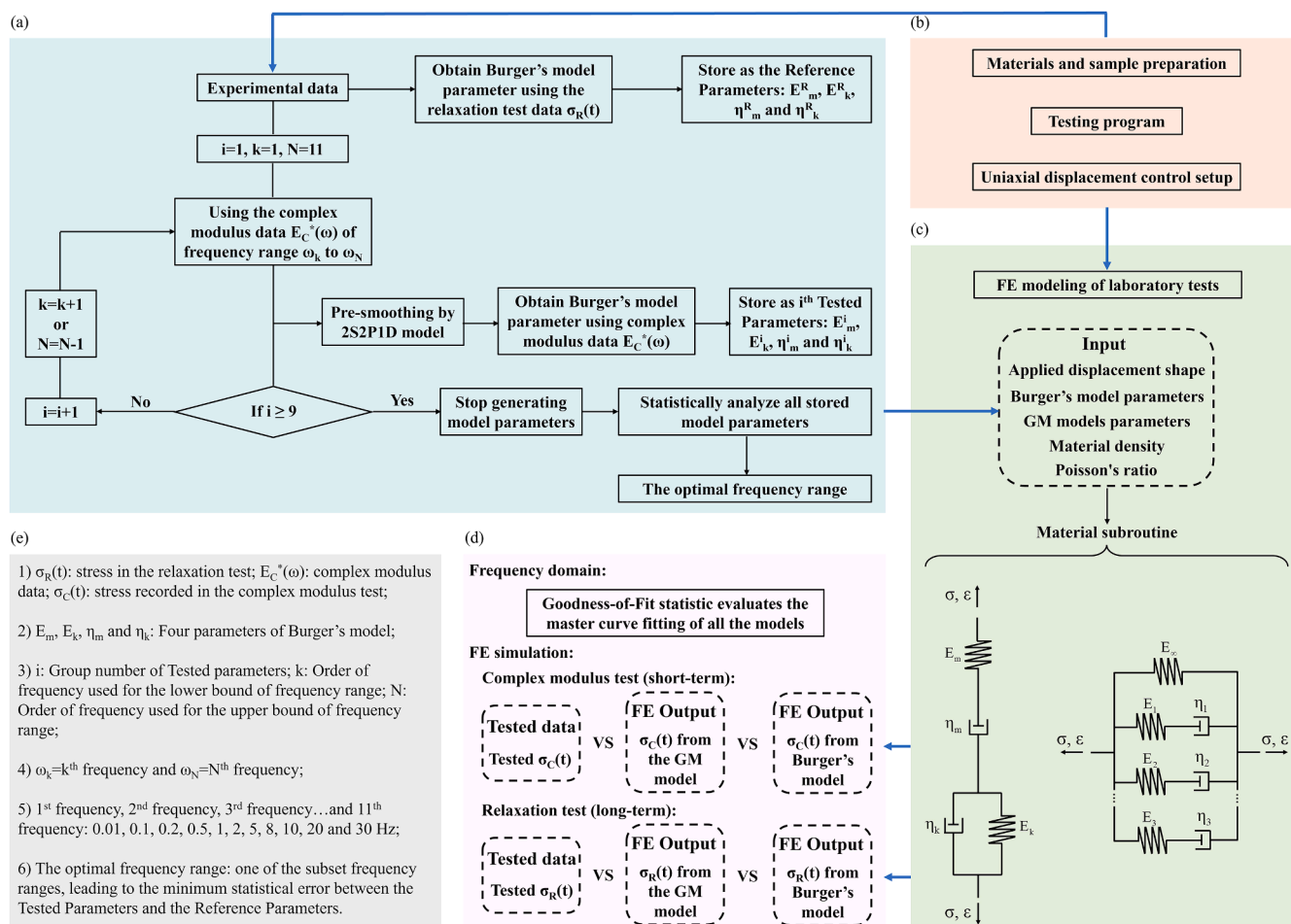
Fig. 1. Overview of research methodology: (a) Proposed framework for determining the optimal frequency range for Burger's model. This subfigure illustrates the process of identifying the optimal frequency subset range, utilizing experimental data from both complex modulus and relaxation tests. Model parameters derived from the relaxation test data serve as reference values, guiding the evaluation of model parameters obtained from complex modulus test data across different subset frequency ranges. Number k and N dictate the frequency data point limits, generating various subset frequency ranges for evaluation. Statistical analysis of all derived model parameters ultimately determines the optimal frequency range. (b) Laboratory tests. Complex modulus and relaxation test data are used as inputs for the proposed framework, while asphalt sample geometry and test conditions inform the FE simulation. (c) FE simulation process. Model parameters from the identified optimal frequency range are the key input to define the material's linear viscoelastic properties. Two material model subroutines are implemented within the FE software. (d) Performance evaluation of Burger's Model in both frequency and time domains, comparing FE simulation results with test results. (e) Nomenclature and additional explanations related to terms and processes in the methodology.
