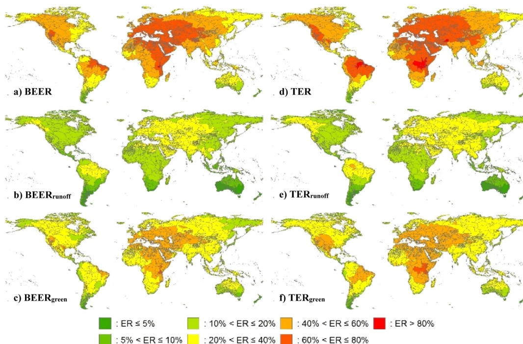
Figure 3. Basin-specific ER ratios for the basin external inventory (a–c) and across all basin boundaries (d–f) averaged over the year; (a) BEER, (b) runoff-relevant BEER (BEER runoff ), (c) green water-relevant BEER (BEER green ), (d) TER, (e) runoff-relevant TER (TER runoff ), and (f) green water-relevant TER (TER green ).
