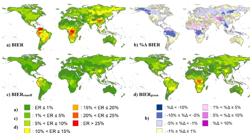
Figure 2. Basin-specific ER ratios for the basin internal inventory perspective averaged over the year (a) BIER, (b) total percentage changes (%Δ) of the updated BIER ratios in comparison to those of the previous WAVE+ publication, (c) runoff-relevant BIER (BIER runoff ), and (d) green water-relevant BIER (BIER green ).
