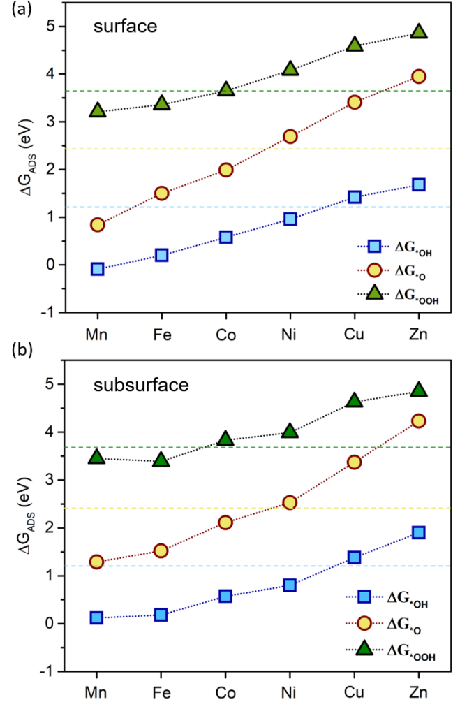
Figure 6. Gibbs free energies of the OER intermediates on TM doped and pristine ZnO (10 \bar{1} 0) (a) surface and (b) subsurface. Adsorbed species are abbreviated as ADS and signifies *OH (blue squares), *O (yellow circles), and *OOH (green triangles). The blue, yellow, and green dashed horizontal lines stand for the Gibbs free energies 1.23, 2.46, and 3.69 eV, respectively.
