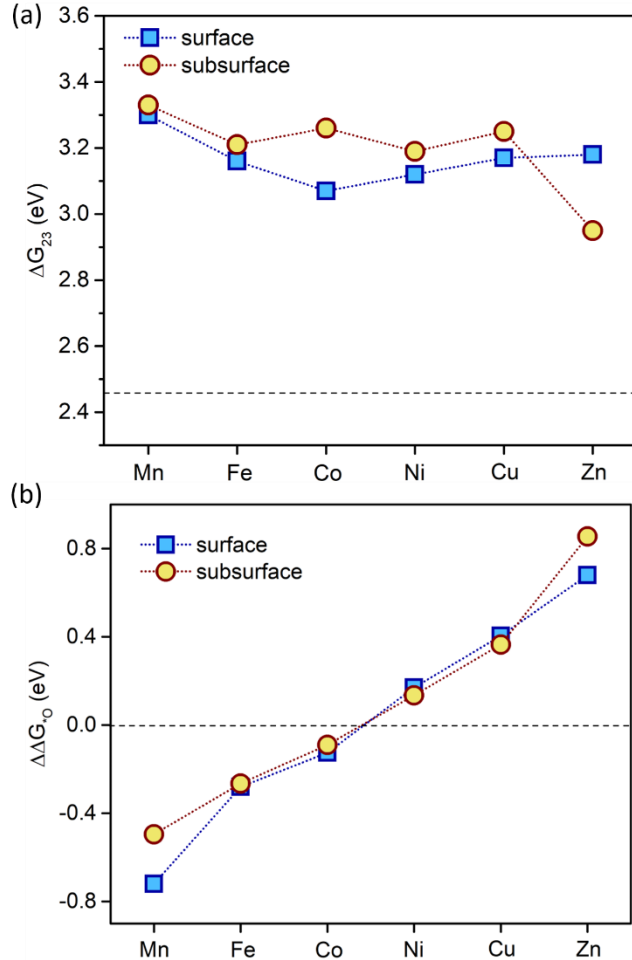
Figure 7. (a) The Gibbs free energy difference \Delta G_{23} on TM doped and pristine ZnO (10 \bar{1} 0) surface and subsurface; the dashed horizontal line indicates the ideal value of 2G_0 = 2.46 eV. (b) The Gibbs free energy difference \Delta\Delta G_{-O} on TM doped and pristine ZnO (10 \bar{1} 0) surface and subsurface; the value larger than 0 eV indicates weak O adsorption and smaller than 0 eV indicates strong O adsorption; the dashed horizontal line indicates the optimal value of 0 eV. The lines between data points are added to guide the eye.
