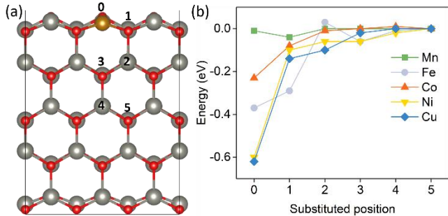
Figure 2. (a) Side view of the substituted positions of the TM in ZnO (10 \bar{1} 0) surface, (b) total energy in different substituted positions, the x axis indicates the substituted position. We assume the total energy of TM substitutes in the bulk (i.e. substituted position 5) as 0, negative values mean that other substitutions show lower total energy than TM substitutes in the bulk, which are more stable than position 5 substitution.
