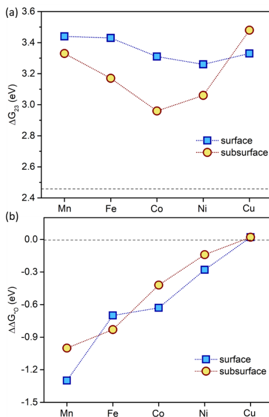
Figure 10. (a) The Gibbs free energy difference \Delta G_{23} on double TMs doped ZnO (10 \bar{1} 0) surface and subsurface; the dashed horizontal line indicates the ideal value of 2G_0 = 2.46 eV. (b) The Gibbs free energy difference \Delta \Delta G_{*O} on double TMs doped ZnO (10 \bar{1} 0) surface and subsurface; the value larger than 0 eV
