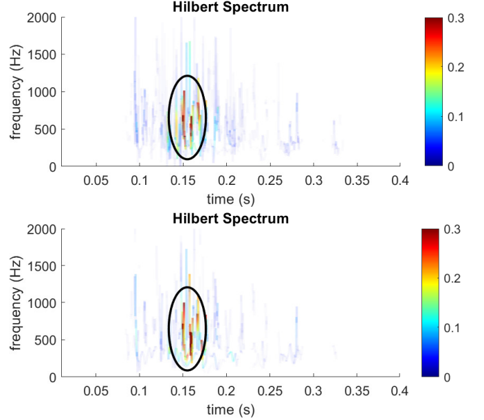
Fig. 5. Top panel: Hilbert spectrum of IMFs by projection on the generalized eigenspace for eigenvalue 0 of Q . Bottom panel: Hilbert spectrum of IMFs by the classic EMD.
