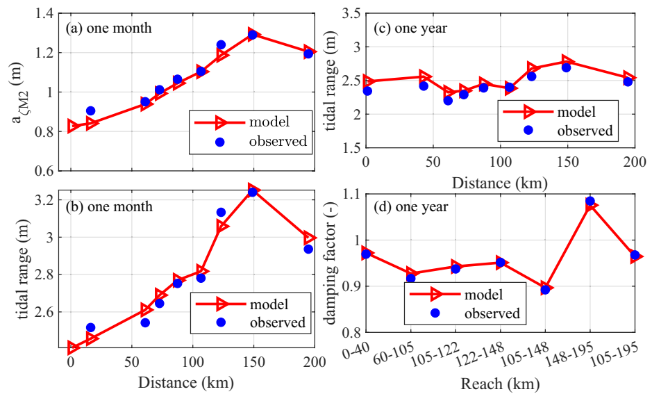
Figure 3. Comparison between observed and modeled (a) M_2 amplitude ( a_{M2} ) during 15 August–September 15, 2007; (b) tidal range during 15 August–September 15, 2007; (c) yearly averaged tidal range in 2007; and (d) yearly averaged damping factor in the reaches Xuliujing–Yanglin (0–40 km), Shidongkou–Hengsha (60–105 km), Hengsha–Beicaozhong (105–122 km), Beicaozhong–Niupijiao (122–148 km), Hengsha–Niupijiao (105–148 km), Niupijiao–Lvhu (148–195 km), and Hengsha–Lvhu (105–195 km) in 2007.
