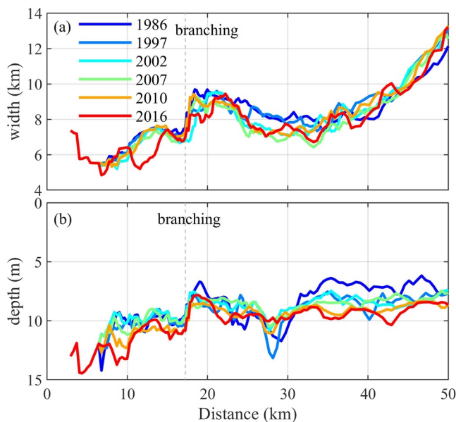
Figure 8. Longitudinal changes of (a) cross-sectional averaged width between high and low water levels and (b) cross-sectional averaged water depth in 1986, 1997, 2002, 2007, 2010, and 2016. The “branching” indicates the location where the bifurcation between the North Branch and South Branch starts.
