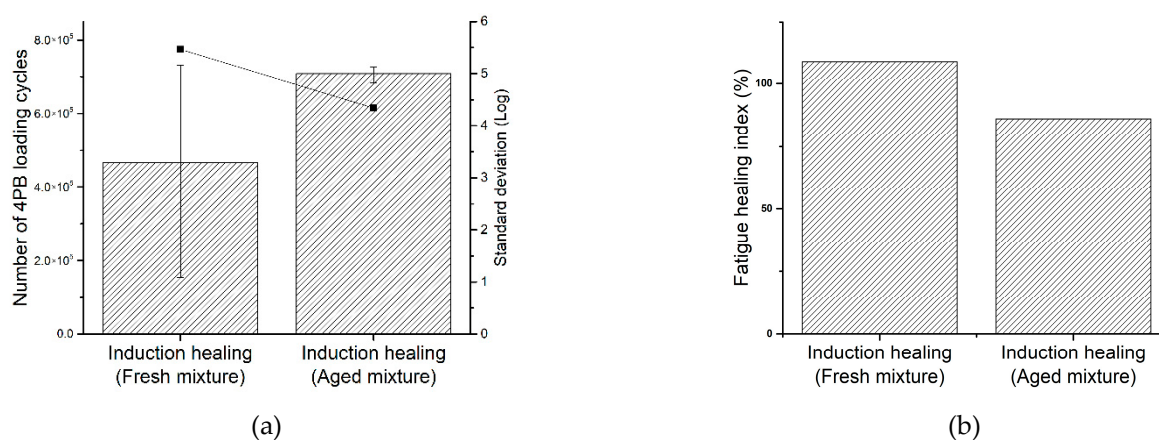
Figure 14. Four-point bending fatigue test results for the induction healing system in PA mixture with different ageing levels: (a) total number of 4PB fatigue loading cycles and (b) the fatigue healing index.
