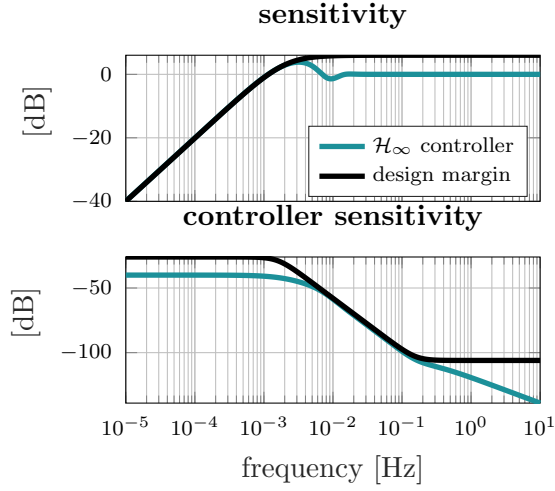
Figure 7. The performance evaluation of the designed controller: The sensitivity \mathcal{S} and the controller sensitivity \mathcal{U} . The design margins calculated from the performance weights are shown in black.
