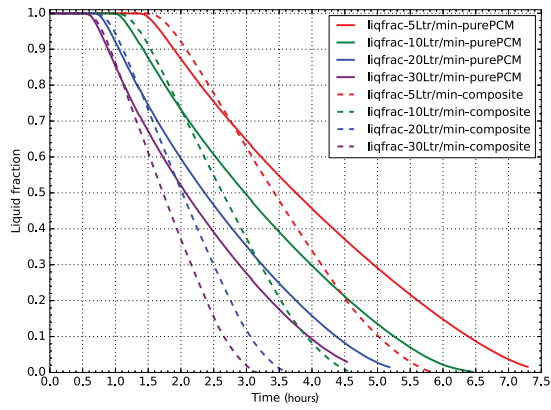
(a) Liquid fraction with varying air flow rate
