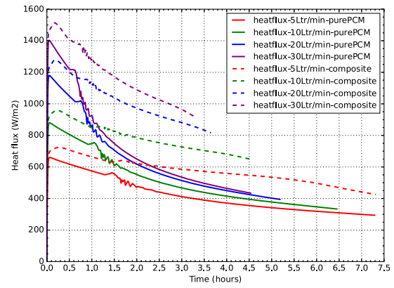
(b) Heat flux with varying air flow rate
