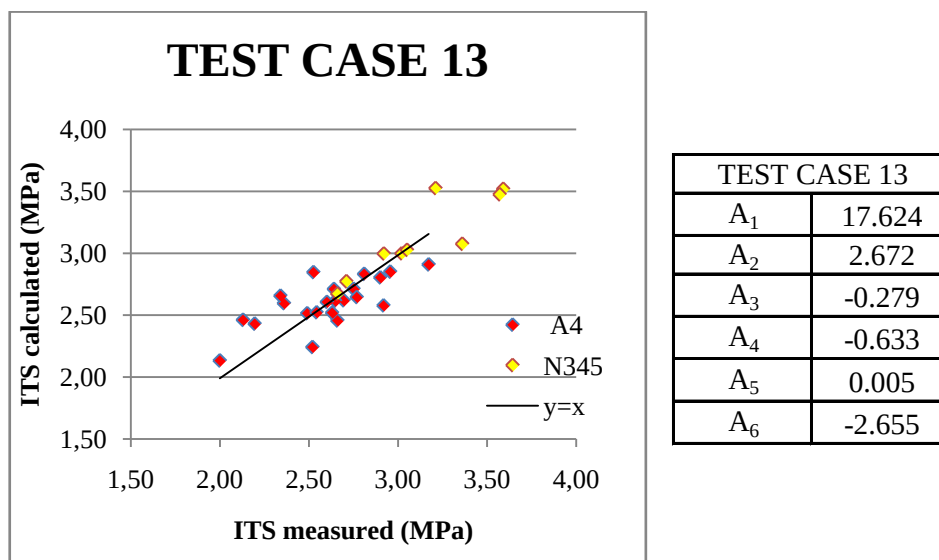
FIGURE 3 Test case 13 Measured and calculated ITS; multipliers.
