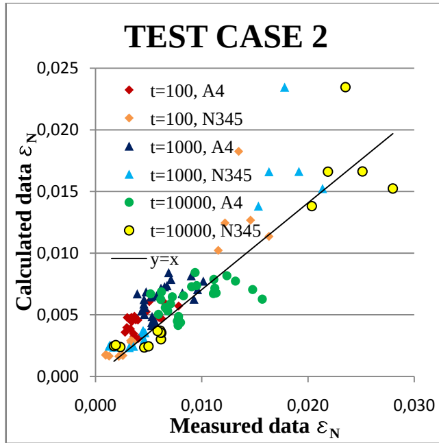
FIGURE 6 Test case 2 Measured and calculated \varepsilon_N ; multipliers.
