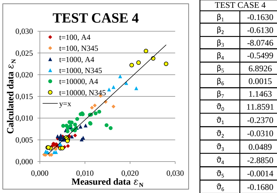
FIGURE 8 Test case 4 measured and calculated \varepsilon_N ; multipliers.
