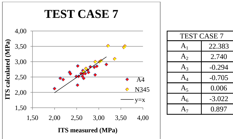
FIGURE 2 Test case 7 Measured and calculated ITS; multipliers.
