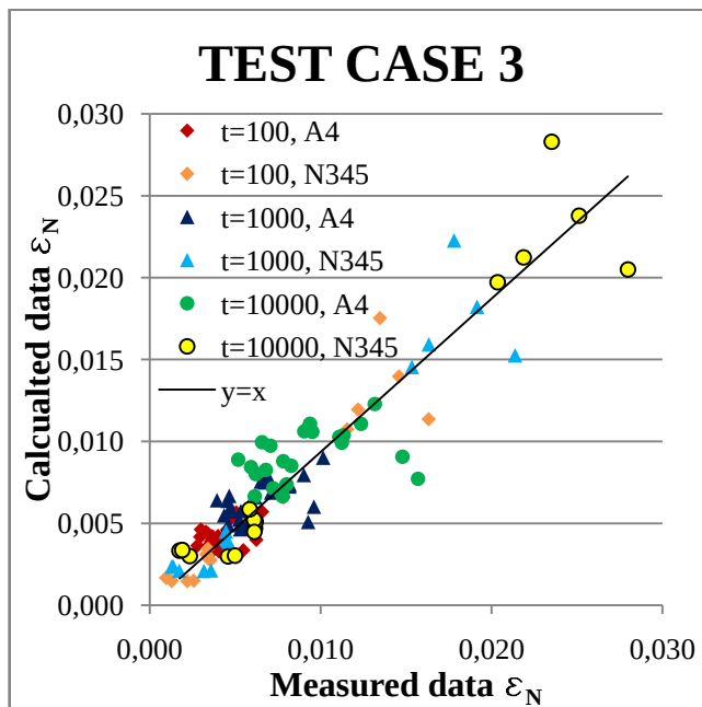
FIGURE 7 Test case 3 measured and calculated \varepsilon_N ; multipliers.
