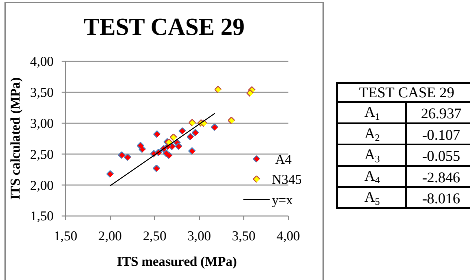
FIGURE 4 Test case 29 Measured and calculated ITS; multipliers.
