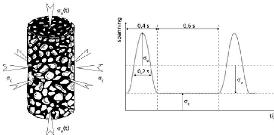
FIGURE 1 Schematic of the stress signal in time.
