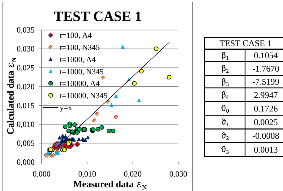
FIGURE 5 Test case 1 Measured and calculated \varepsilon_N ; multipliers.
