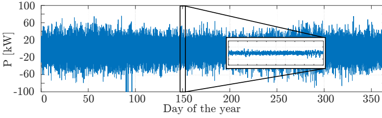
Figure 4.15: Yearly mission profiles of a 100 kW 2L-VSC used as grid interface for a BESS providing frequency regulation, with zoom in one day.
