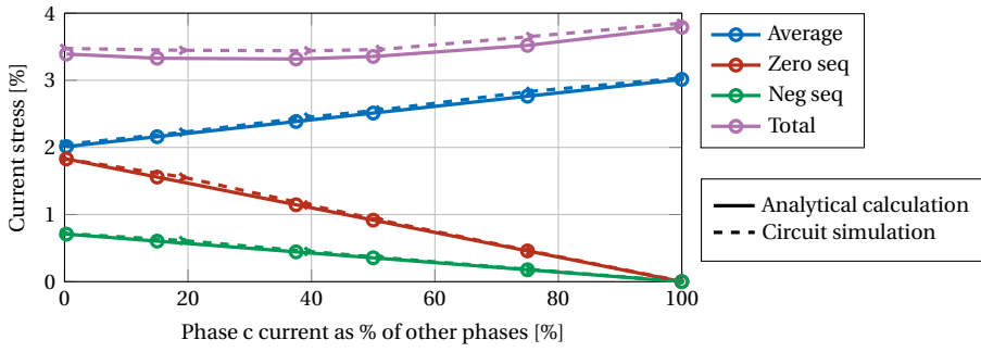
Figure 5.5: Total rms current in the DC-link and its various components, when I_a and I_b are equal to 3.7A and I_c is varied from 0 to 3.7A. Both the analytically calculated values through (5.6)-(5.9), and the ones derived from the circuit simulator PLECS are reported.
