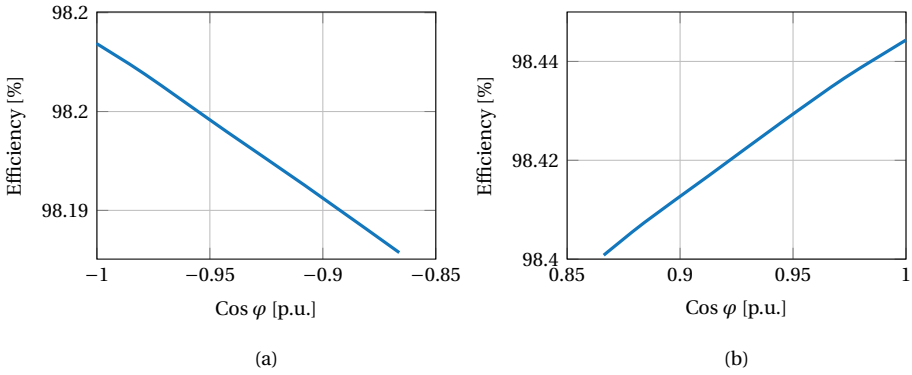
Figure 4.14: Semicondutor efficiency of a mcHyS-based 2L-VSC designed as (a) inverter and (b) rectifier operating at rated apparent power and varying the power factor.
