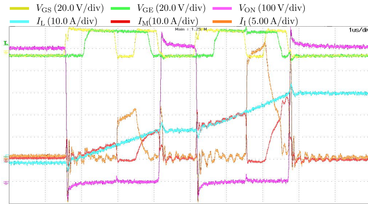
Figure 4.6: Double Pulse Test waveforms of mHyS obtained through the test setup of Figure B.1 and referred to the circuit schematic of Figure B.2 (a).
