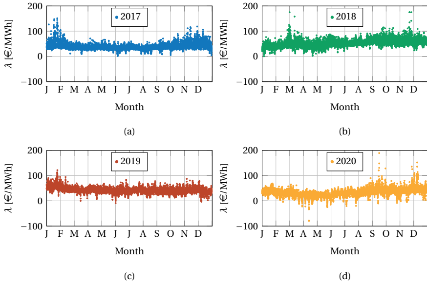
Figure 6.5: Scattered plot of the dutch DAM market prices from 2018 to 2020 plotted in a single year roll-out.
