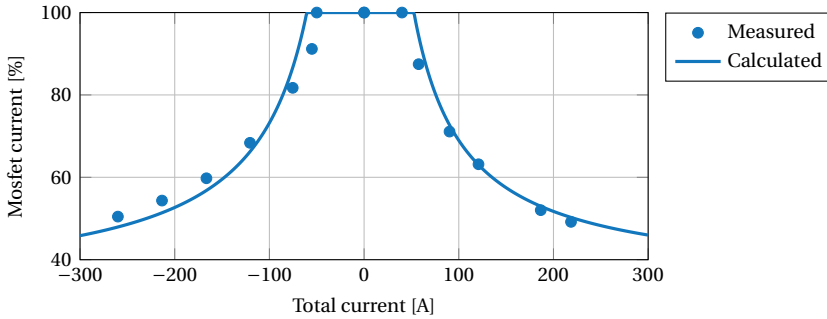
Figure 4.4: Percentage of the total conducted current by the tHyS flowing through the MOSFET channel; derived for T_j=25^\circ\text{C} , V_{gs} and V_{ge}=+17/-4\text{ V} , and R_g=4\Omega , and analytically calculated according to (A.17) and (A.19).
