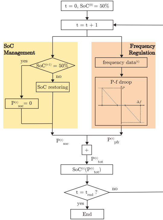
Figure 3.3: Flowchart describing the algorithm for PFR provision, where t indicates the time instant and P_{\text{pfr}}^t and P_{\text{SoC}}^t are respectively the frequency regulation power and the SoC control power at the instant t .
