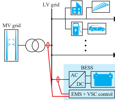
Figure 5.1: Example of a LV distribution grid where unbalanced loads are connected in the LV side and a BESS acts as power redistributor balancing the MV currents.
