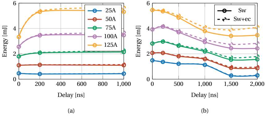
Figure 4.7: HySs turn on (a) and off (b) switching energies (sw) and extra conduction (ec) losses varying the switched current and the MOSFET-IGBT delays d_1 and d_4 .
