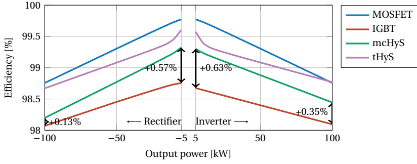
Figure 4.13: Semicondutor efficiency of the switch configurations of Figure 4.13 varying the output power operating as inverter and rectifier 2L-VSCs. The selected designs are shown in Figure 4.12 and represent the chip area optimized for minimal cost.
