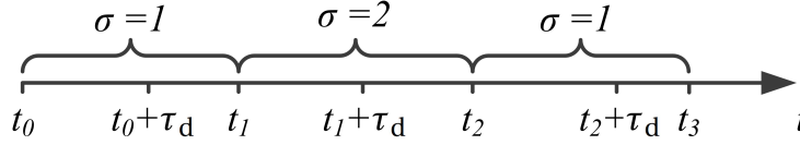
Figure 2.4: A dwell time switching signal.
