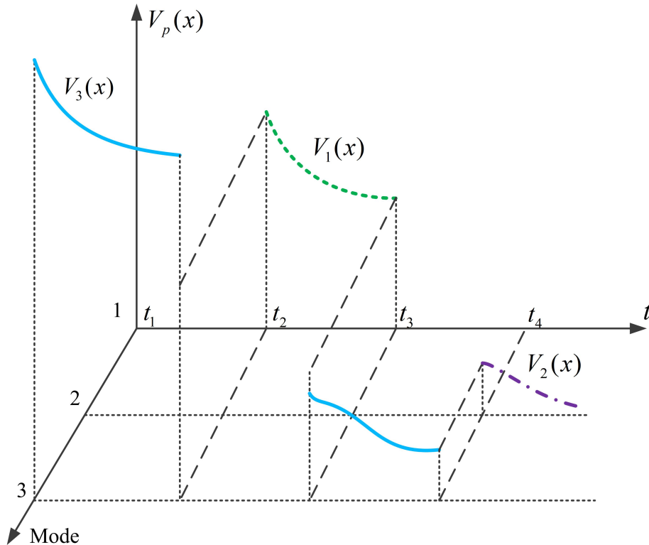
Figure 2.3: Stability condition II: when switching subsystem 3 to subsystem 1 at the switching instant t_2 , the value of its corresponding Lyapunov function V_1(t_2) is smaller than the value of the Lyapunov function V_3(t_1) of subsystem 3.
