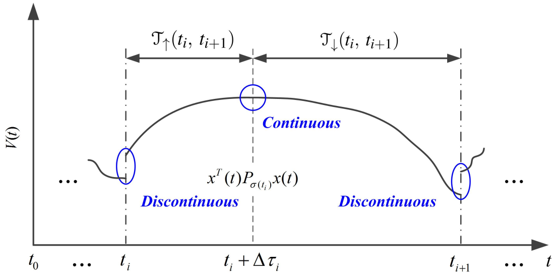
Figure 7.1: The Lyapunov function (7.6).
