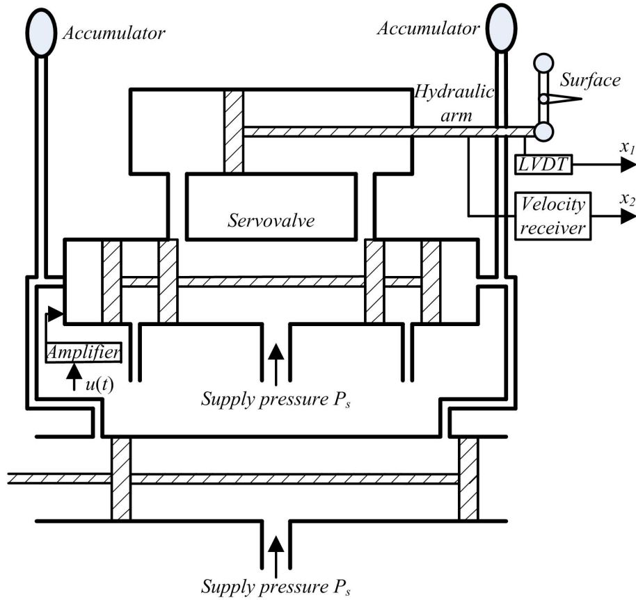
Figure 4.2: The schematic diagram of the electro-hydraulic system.
