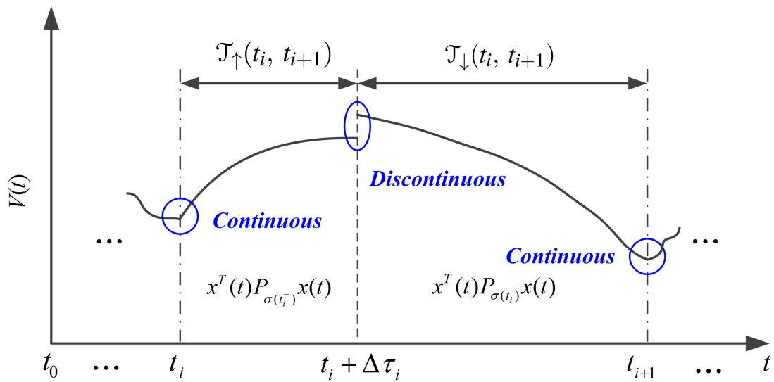
Figure 7.2: The proposed Lyapunov function (7.7).
