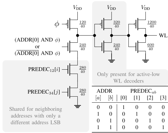
Fig. 2. Row decoder schematic, including transistor (W/L) in nm and the 2-bit predecoder truth table. The optional inverter in gray is only included for the row decoders where the active WL is low, i.e., overlined WWL and RWLs in Fig. 1.
