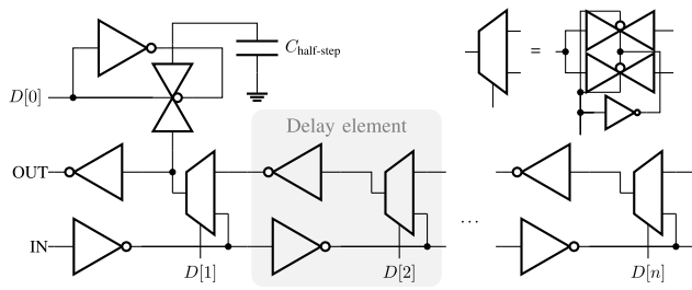
Fig. 5. Delay chain used to generate the timing for the memory control signals. The (W/L) of all transistors is (300 nm/40 nm) and (500 nm/40 nm) for NMOS and PMOS, respectively, except for the transistors in the inverters driving the transmission gates, which are minimum-sized (120 nm/40 nm).
