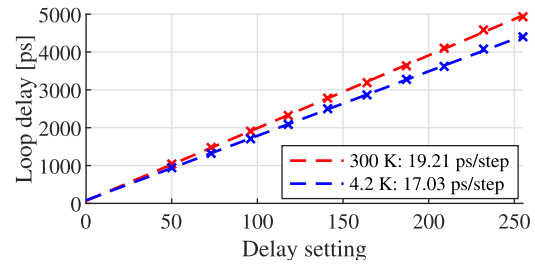
Fig. 9. RO loop delay as a function of the delay chain settings with a least-squares linear fit ( V_{DD} = 1.1 \text{ V} ).
