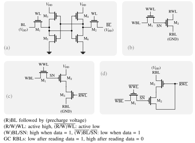
Fig. 1. Schematics of the four cell designs: (a) 6T static cell; (b) 2T NW-PR dynamic gain cell; (c) 3T NW-PR dynamic gain cell; and (d) 3T PW-PR preferentially boosted dynamic gain cell. The readout current of the dynamic cells always flows from top to bottom.
