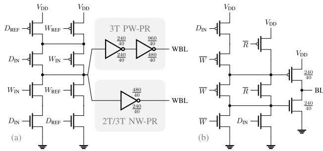
Fig. 4. BL driver for: (a) dynamic memories and (b) static memories with transistor (W/L) sizes in nm. In (a), unannotated transistors are minimum-sized (W/L = 120/40) and inverter PMOS/NMOS sizes are shown above/below the inverters, respectively; the driving inverters in the gray boxes are alternatively used for the respective memory. In (b), unannotated NMOS transistors are minimum-sized (W/L = 120/40) while unannotated PMOS transistors are double-width, minimum-length (W/L = 240/40).
