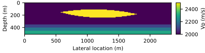
Figure 4.7: Model with high velocity perturbation.
