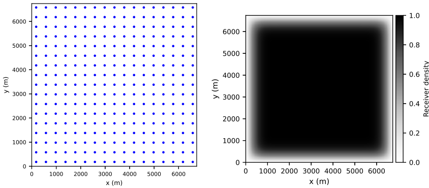
Figure 4.15: (a) Initial uniform receiver geometry and (b) receiver density for the model in Figure 4.14
