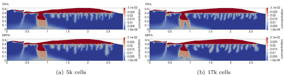
Fig. 9 Resolution study for the model cut in reservoir conditions. The comparison of the spatial distributions of \text{CO}_2 concentration after 15 days was obtained with TPFA and MPFA schemes
